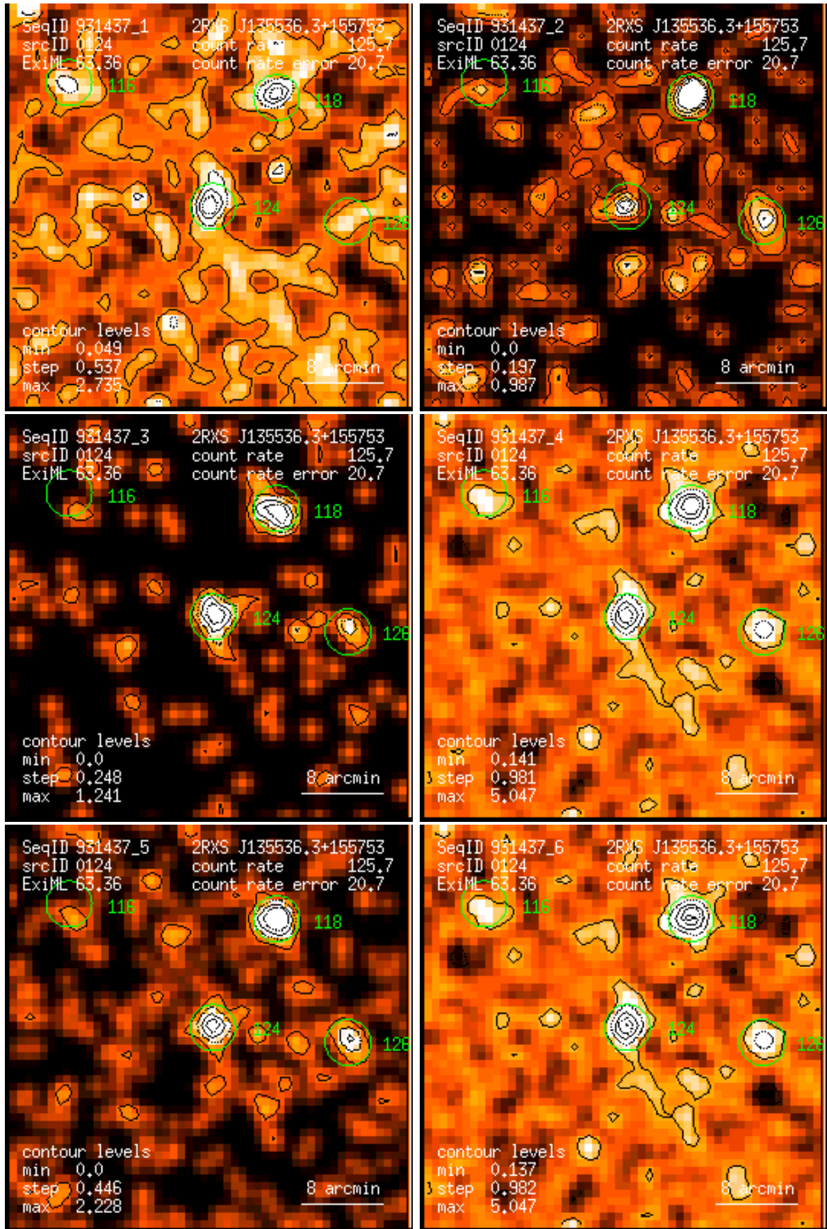
Figure 124: RASS 931437: detection 0124: band rate images, Gaussian filter: (1) PSPC channels 11 – 41, (2) 52 – 90, (3) 91 – 201, (4) 11 – 235, (5) 52 – 201, (6) 11 – 201. Broad band rates in counts/ks. Band rate contour levels in counts/ks/arcmin 2 .
