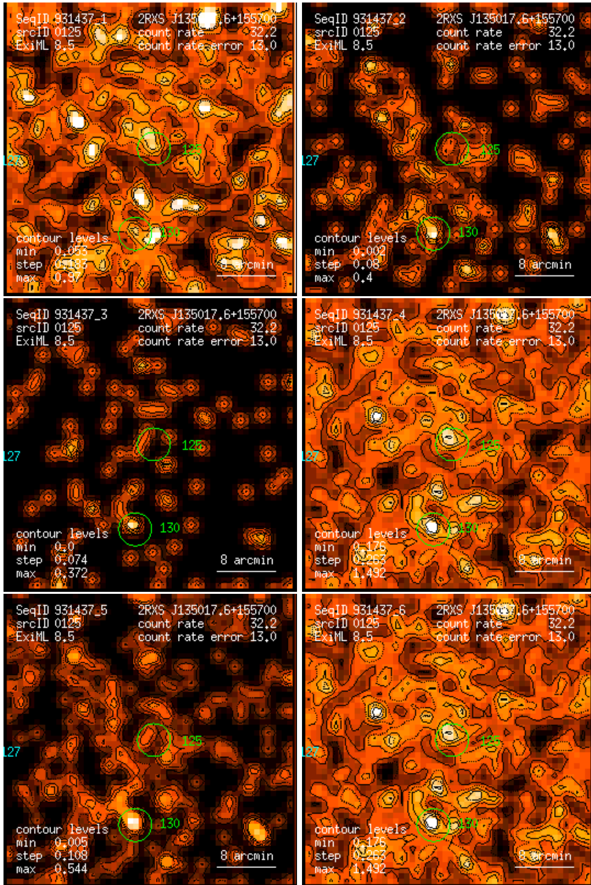
Figure 125: RASS 931437: detection 0125: band rate images, Gaussian filter: (1) PSPC channels 11 – 41, (2) 52 – 90, (3) 91 – 201, (4) 11 – 235, (5) 52 – 201, (6) 11 – 201. Broad band rates in counts/ks. Band rate contour levels in counts/ks/arcmin 2 .
