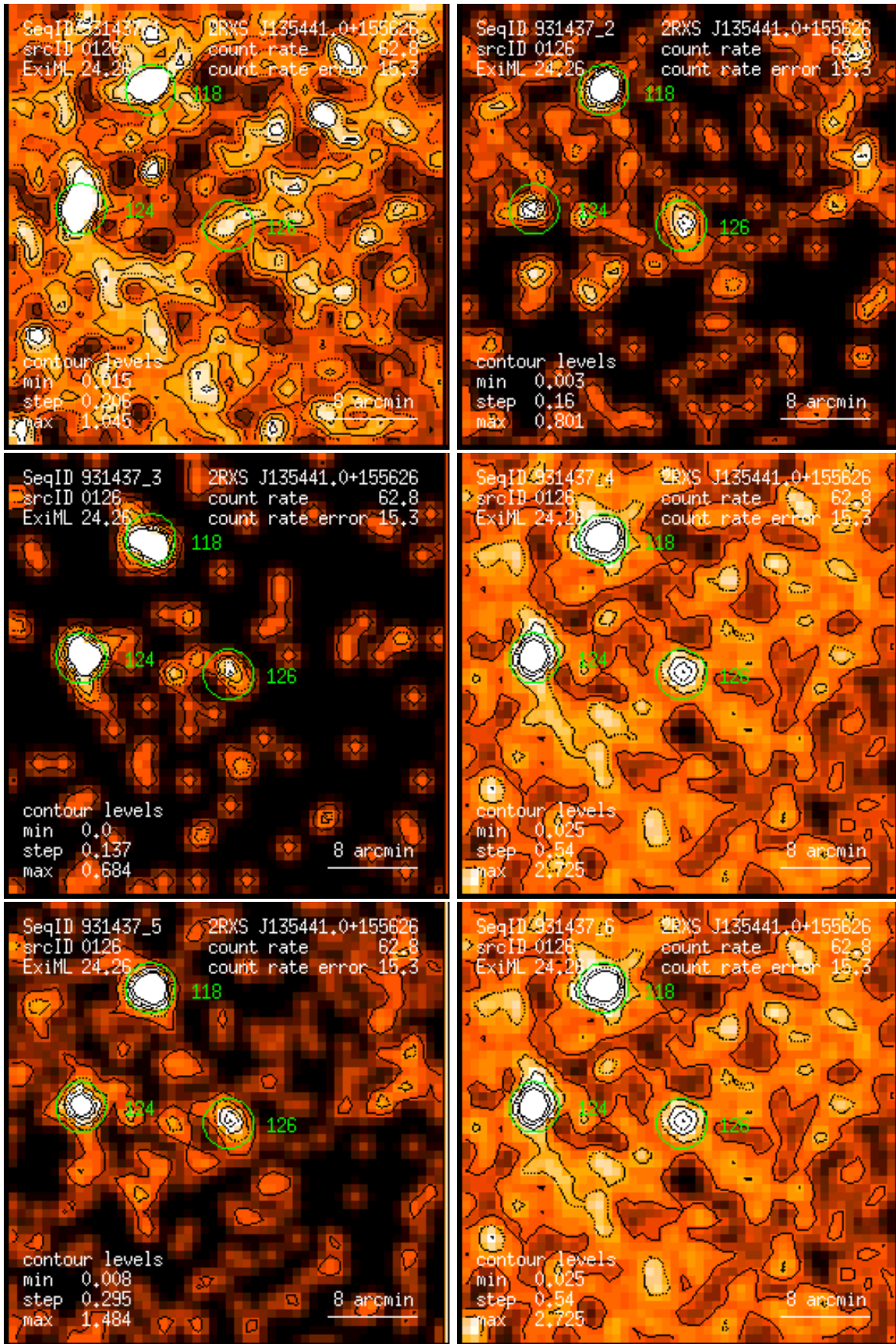
Figure 126: RASS 931437: detection 0126: band rate images, Gaussian filter: (1) PSPC channels 11 – 41, (2) 52 – 90, (3) 91 – 201, (4) 11 – 235, (5) 52 – 201, (6) 11 – 201. Broad band rates in counts/ks. Band rate contour levels in counts/ks/arcmin 2 .
