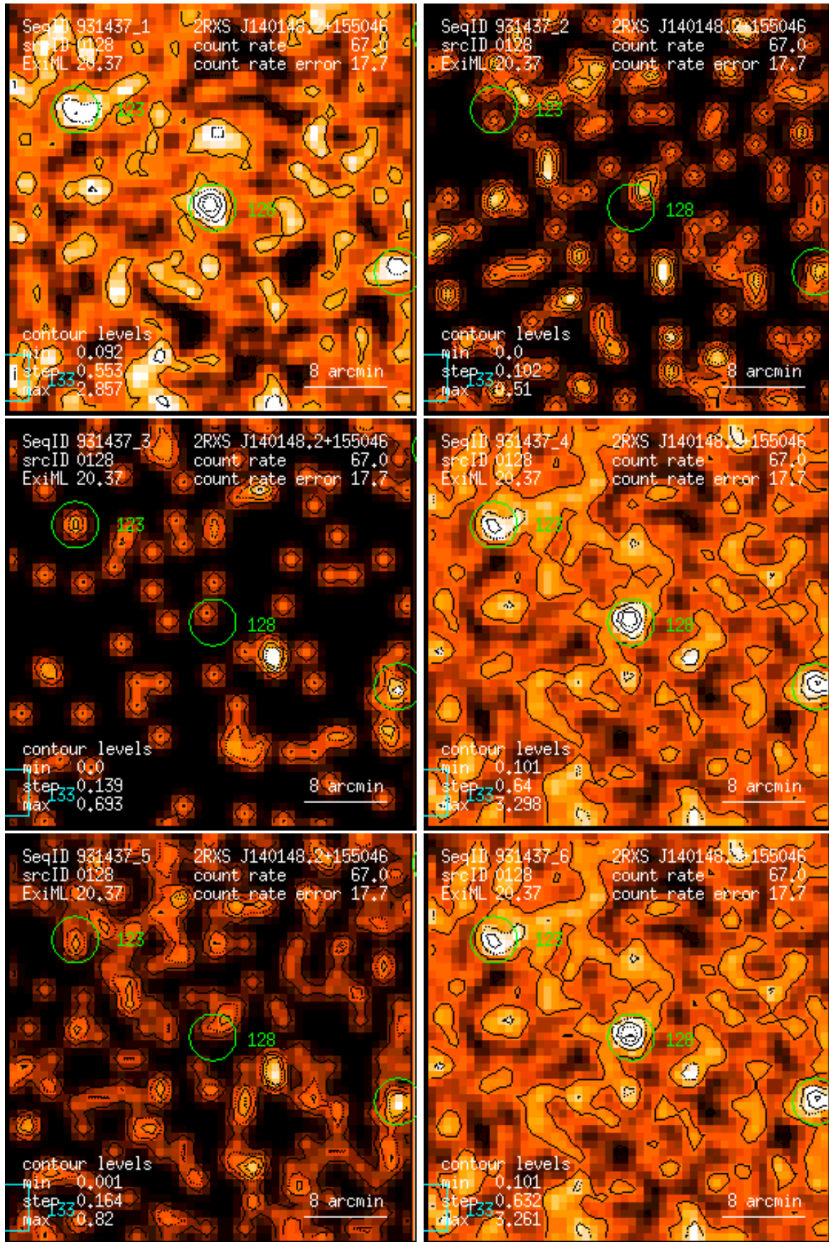
Figure 128: RASS 931437: detection 0128: band rate images, Gaussian filter: (1) PSPC channels 11 – 41, (2) 52 – 90, (3) 91 – 201, (4) 11 – 235, (5) 52 – 201, (6) 11 – 201. Broad band rates in counts/ks. Band rate contour levels in counts/ks/arcmin 2 .
