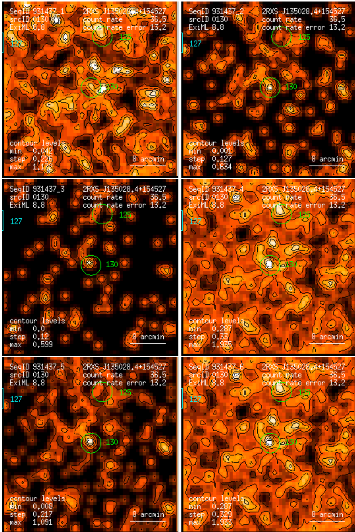
Figure 130: RASS 931437: detection 0130: band rate images, Gaussian filter: (1) PSPC channels 11 – 41, (2) 52 – 90, (3) 91 – 201, (4) 11 – 235, (5) 52 – 201, (6) 11 – 201. Broad band rates in counts/ks. Band rate contour levels in counts/ks/arcmin 2 .
