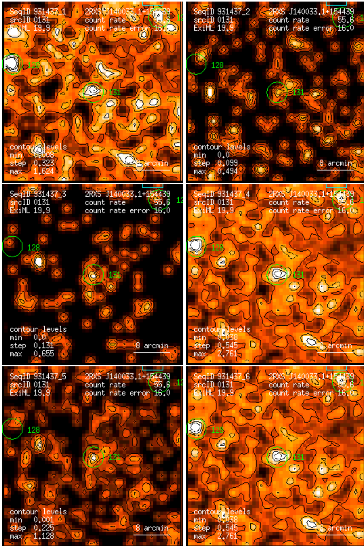
Figure 131: RASS 931437: detection 0131: band rate images, Gaussian filter: (1) PSPC channels 11 – 41, (2) 52 – 90, (3) 91 – 201, (4) 11 – 235, (5) 52 – 201, (6) 11 – 201. Broad band rates in counts/ks. Band rate contour levels in counts/ks/arcmin 2 .
