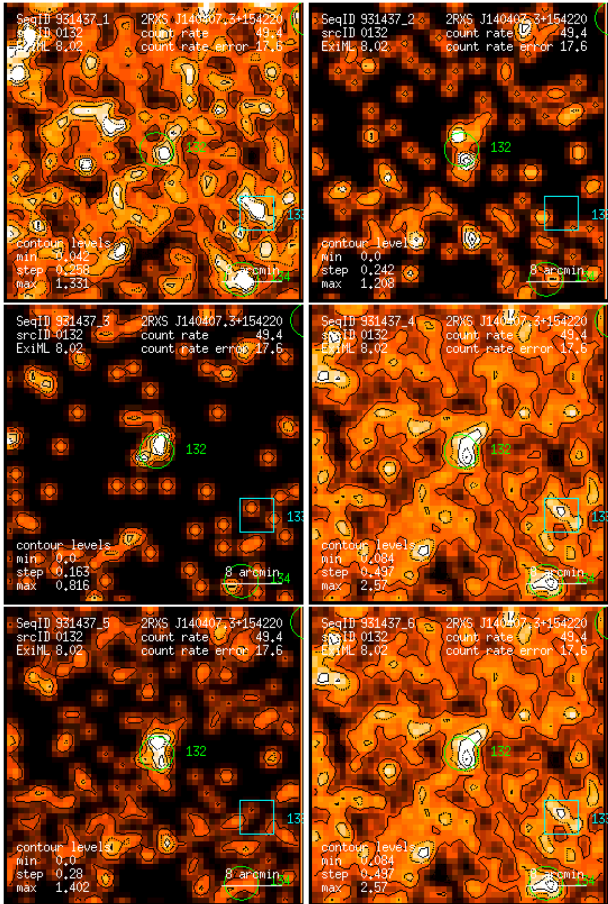
Figure 132: RASS 931437: detection 0132: band rate images, Gaussian filter: (1) PSPC channels 11 – 41, (2) 52 – 90, (3) 91 – 201, (4) 11 – 235, (5) 52 – 201, (6) 11 – 201. Broad band rates in counts/ks. Band rate contour levels in counts/ks/arcmin 2 .
