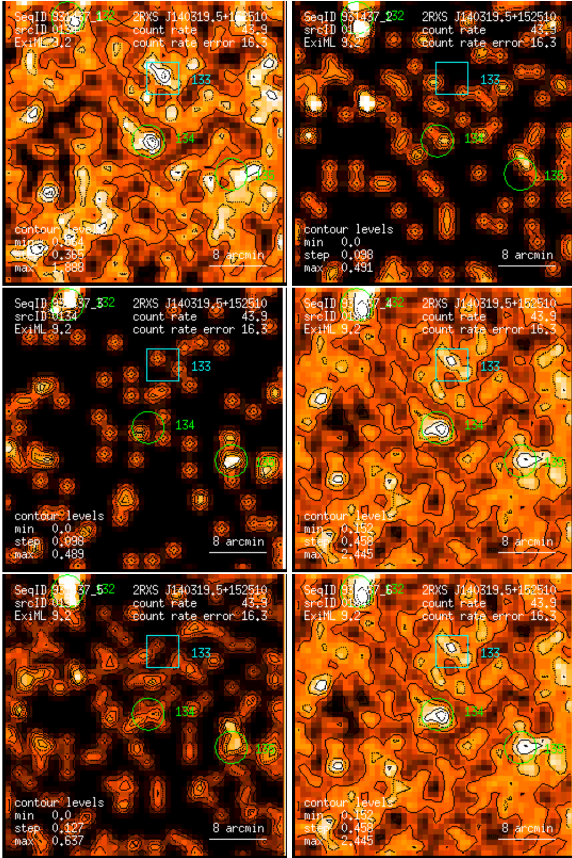
Figure 134: RASS 931437: detection 0134: band rate images, Gaussian filter: (1) PSPC channels 11 – 41, (2) 52 – 90, (3) 91 – 201, (4) 11 – 235, (5) 52 – 201, (6) 11 – 201. Broad band rates in counts/ks. Band rate contour levels in counts/ks/arcmin 2 .
