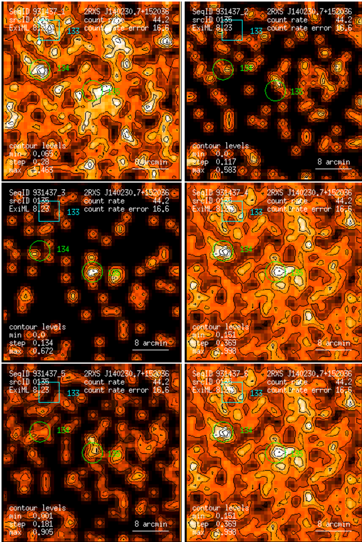
Figure 135: RASS 931437: detection 0135: band rate images, Gaussian filter: (1) PSPC channels 11 – 41, (2) 52 – 90, (3) 91 – 201, (4) 11 – 235, (5) 52 – 201, (6) 11 – 201. Broad band rates in counts/ks. Band rate contour levels in counts/ks/arcmin 2 .
