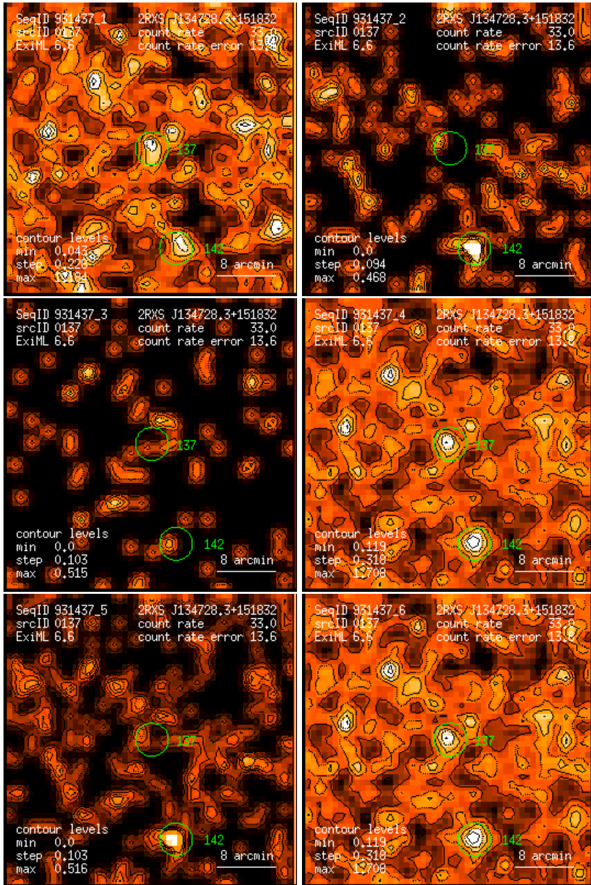
Figure 137: RASS 931437: detection 0137: band rate images, Gaussian filter: (1) PSPC channels 11 – 41, (2) 52 – 90, (3) 91 – 201, (4) 11 – 235, (5) 52 – 201, (6) 11 – 201. Broad band rates in counts/ks. Band rate contour levels in counts/ks/arcmin 2 .
