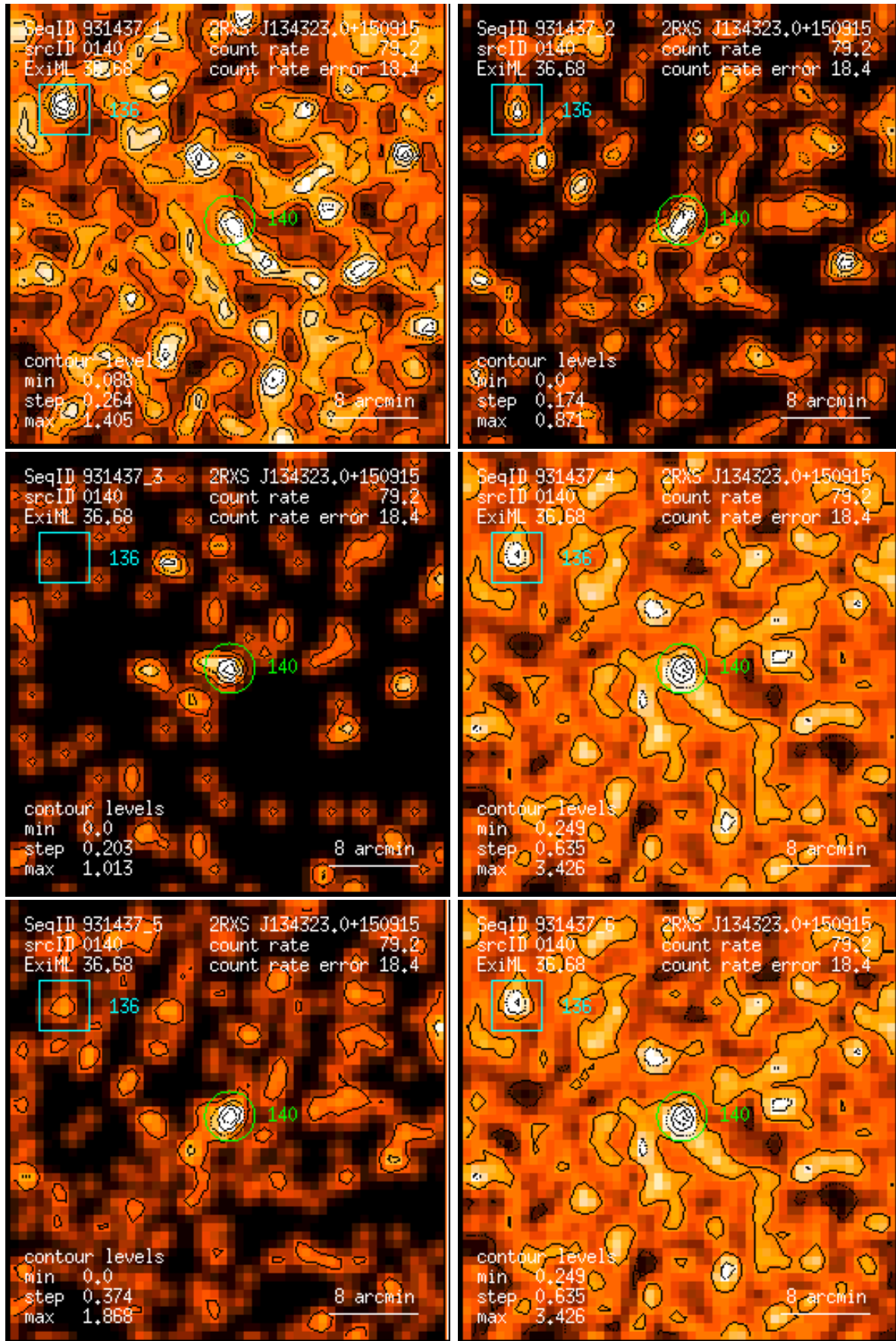
Figure 140: RASS 931437: detection 0140: band rate images, Gaussian filter: (1) PSPC channels 11 – 41, (2) 52 – 90, (3) 91 – 201, (4) 11 – 235, (5) 52 – 201, (6) 11 – 201. Broad band rates in counts/ks. Band rate contour levels in counts/ks/arcmin 2 .
