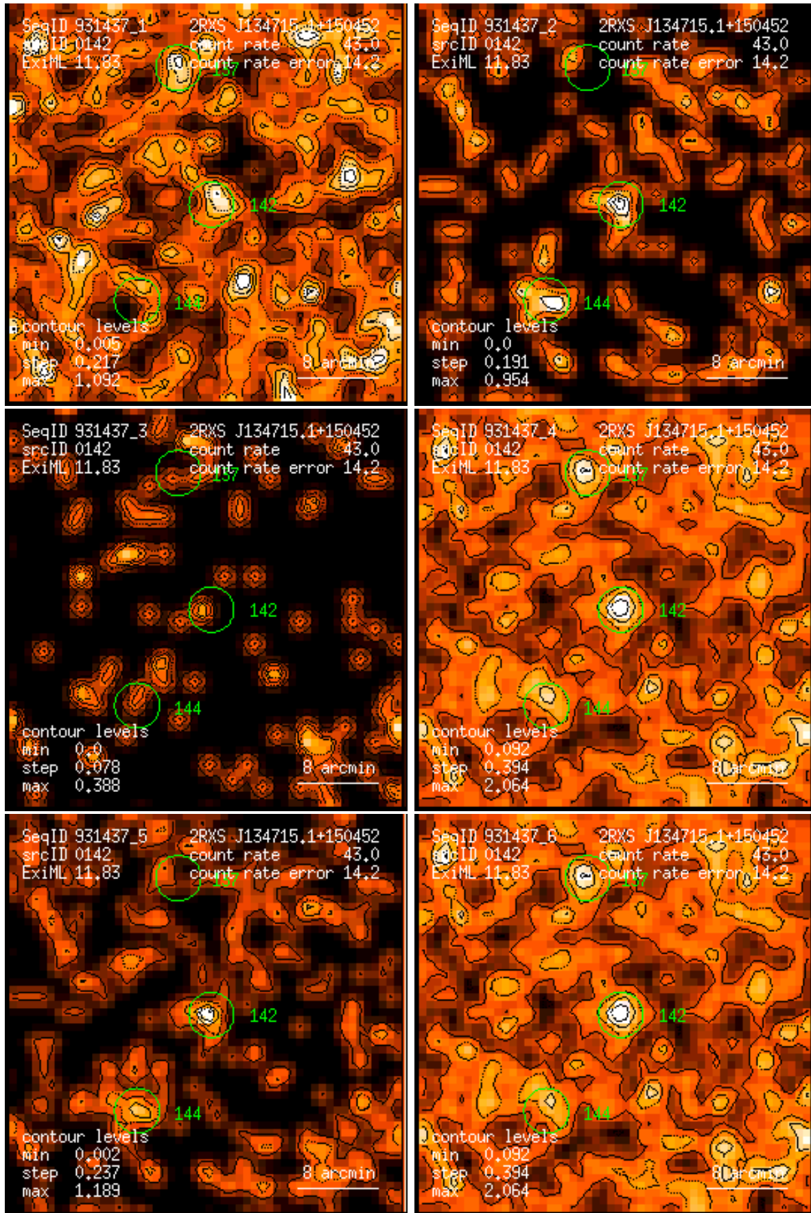
Figure 142: RASS 931437: detection 0142: band rate images, Gaussian filter: (1) PSPC channels 11 – 41, (2) 52 – 90, (3) 91 – 201, (4) 11 – 235, (5) 52 – 201, (6) 11 – 201. Broad band rates in counts/ks. Band rate contour levels in counts/ks/arcmin 2 .
