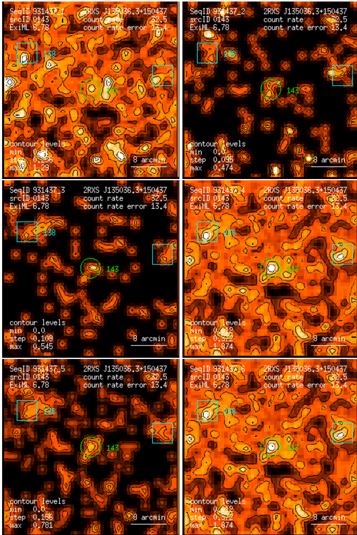
Figure 143: RASS 931437: detection 0143: band rate images, Gaussian filter: (1) PSPC channels 11 – 41, (2) 52 – 90, (3) 91 – 201, (4) 11 – 235, (5) 52 – 201, (6) 11 – 201. Broad band rates in counts/ks. Band rate contour levels in counts/ks/arcmin 2 .
