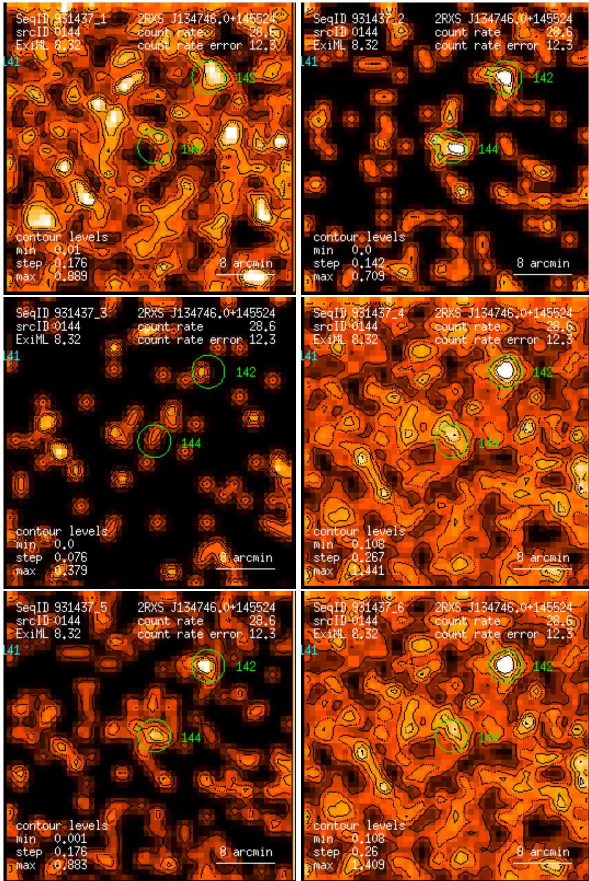
Figure 144: RASS 931437: detection 0144: band rate images, Gaussian filter: (1) PSPC channels 11 – 41, (2) 52 – 90, (3) 91 – 201, (4) 11 – 235, (5) 52 – 201, (6) 11 – 201. Broad band rates in counts/ks. Band rate contour levels in counts/ks/arcmin 2 .
