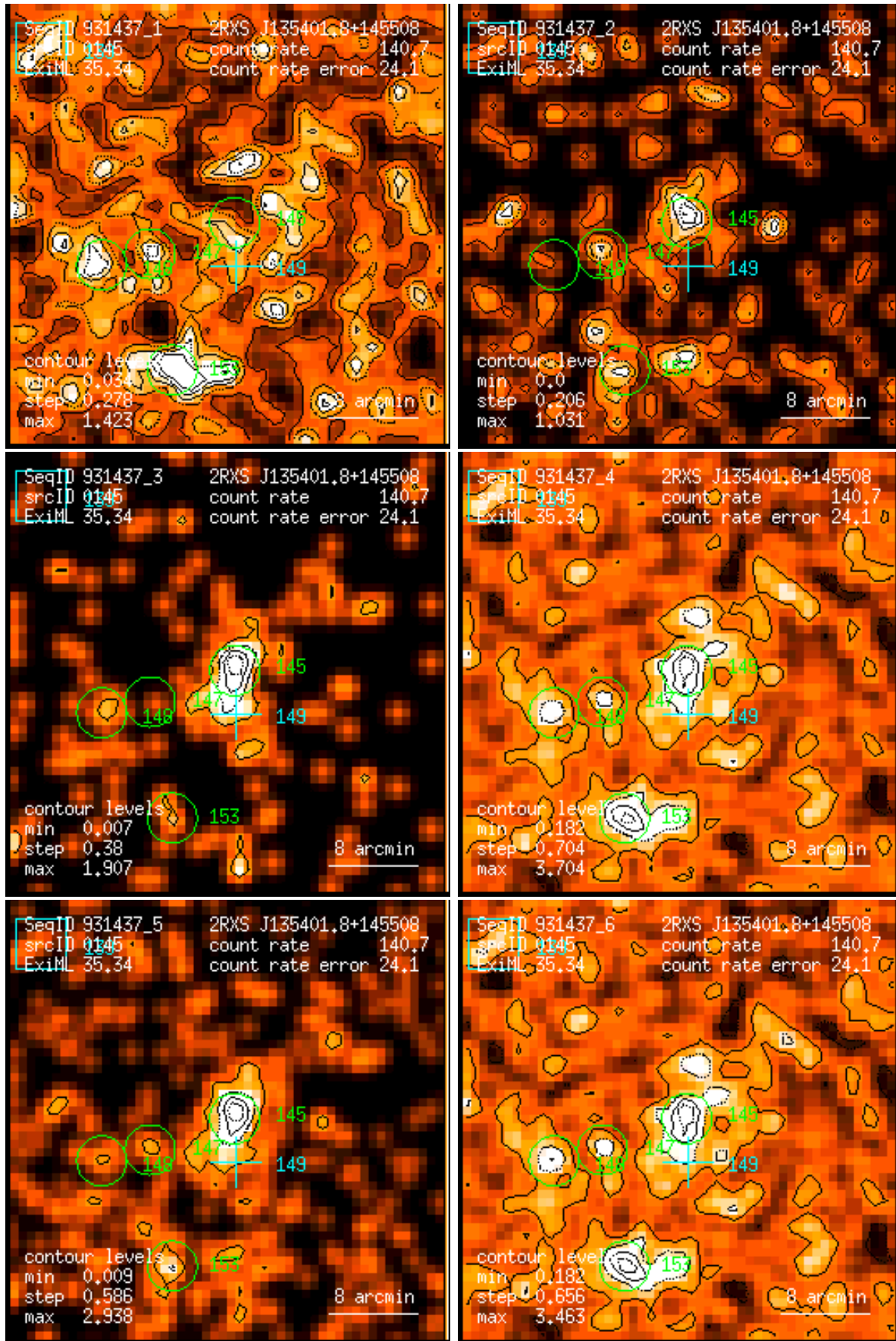
Figure 145: RASS 931437: detection 0145: band rate images, Gaussian filter: (1) PSPC channels 11 – 41, (2) 52 – 90, (3) 91 – 201, (4) 11 – 235, (5) 52 – 201, (6) 11 – 201. Broad band rates in counts/ks. Band rate contour levels in counts/ks/arcmin 2 .
