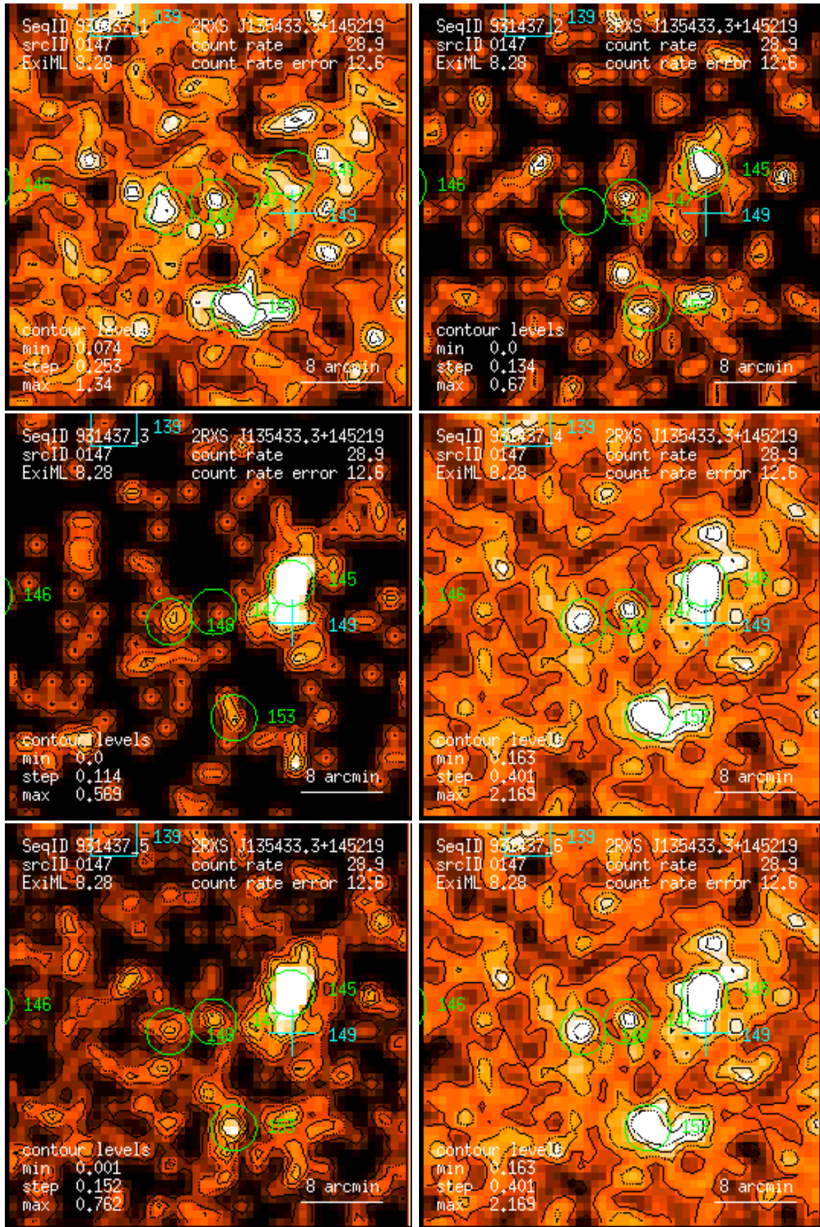
Figure 147: RASS 931437: detection 0147: band rate images, Gaussian filter: (1) PSPC channels 11 – 41, (2) 52 – 90, (3) 91 – 201, (4) 11 – 235, (5) 52 – 201, (6) 11 – 201. Broad band rates in counts/ks. Band rate contour levels in counts/ks/arcmin 2 .
