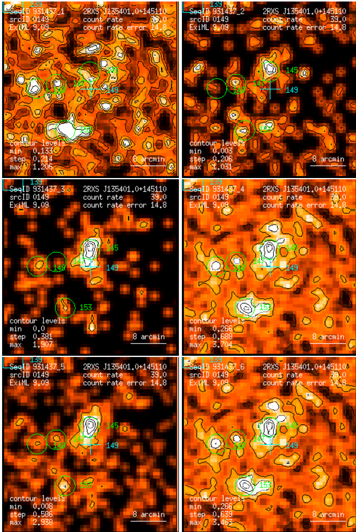
Figure 149: RASS 931437: detection 0149: band rate images, Gaussian filter: (1) PSPC channels 11 – 41, (2) 52 – 90, (3) 91 – 201, (4) 11 – 235, (5) 52 – 201, (6) 11 – 201. Broad band rates in counts/ks. Band rate contour levels in counts/ks/arcmin 2 .
