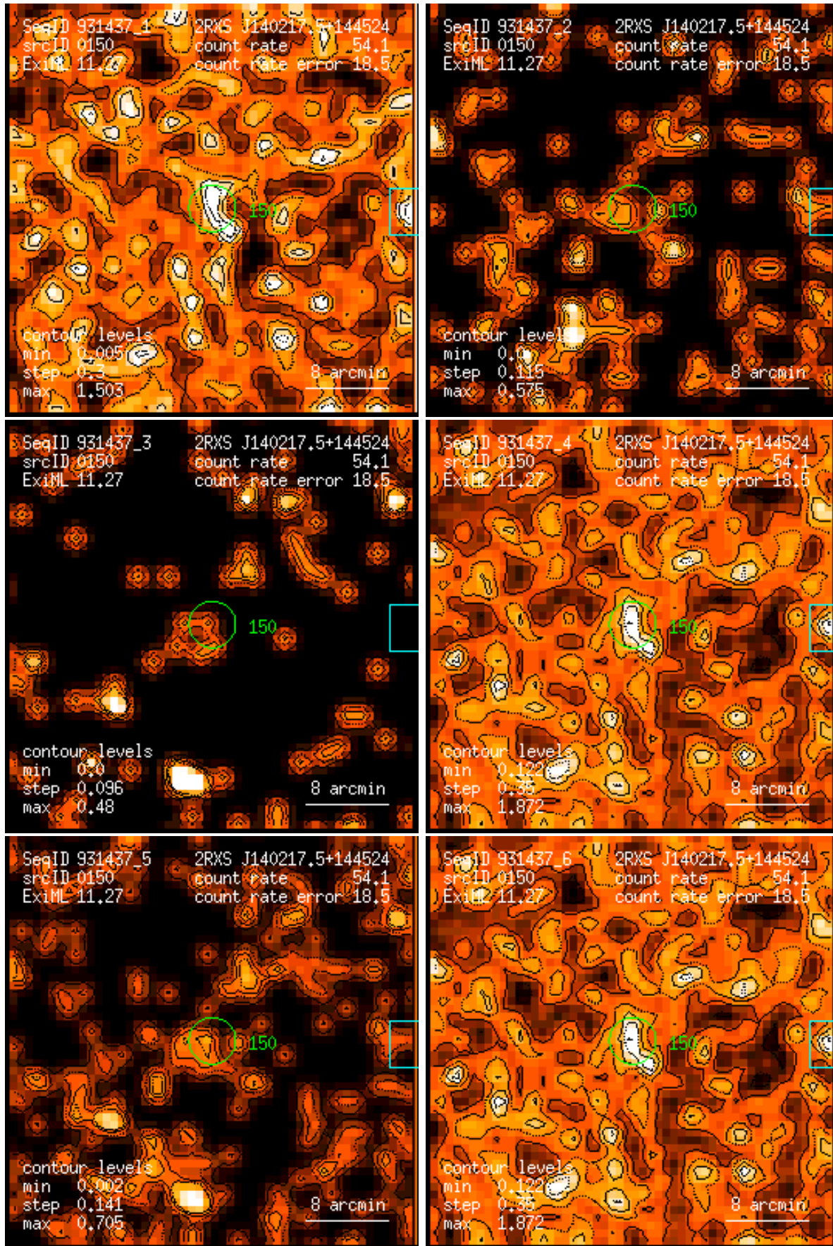
Figure 150: RASS 931437: detection 0150: band rate images, Gaussian filter: (1) PSPC channels 11 – 41, (2) 52 – 90, (3) 91 – 201, (4) 11 – 235, (5) 52 – 201, (6) 11 – 201. Broad band rates in counts/ks. Band rate contour levels in counts/ks/arcmin 2 .
