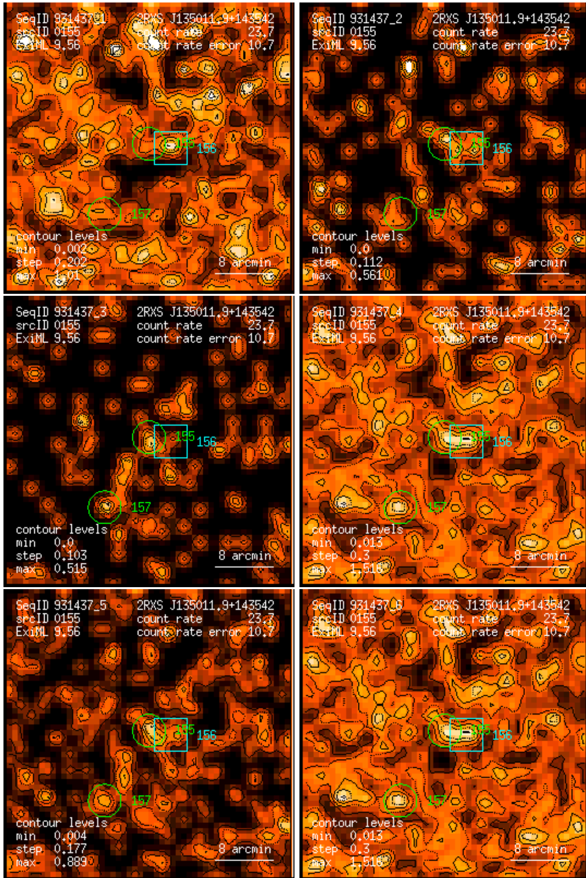
Figure 155: RASS 931437: detection 0155: band rate images, Gaussian filter: (1) PSPC channels 11 – 41, (2) 52 – 90, (3) 91 – 201, (4) 11 – 235, (5) 52 – 201, (6) 11 – 201. Broad band rates in counts/ks. Band rate contour levels in counts/ks/arcmin 2 .
