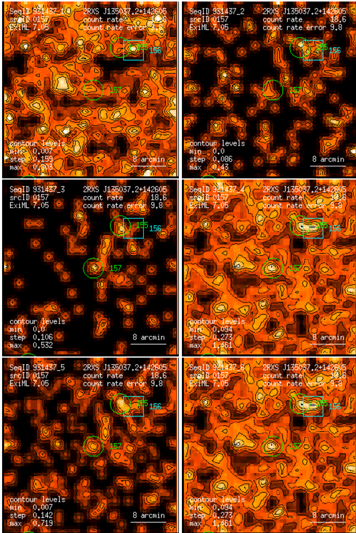
Figure 157: RASS 931437: detection 0157: band rate images, Gaussian filter: (1) PSPC channels 11 – 41, (2) 52 – 90, (3) 91 – 201, (4) 11 – 235, (5) 52 – 201, (6) 11 – 201. Broad band rates in counts/ks. Band rate contour levels in counts/ks/arcmin 2 .
