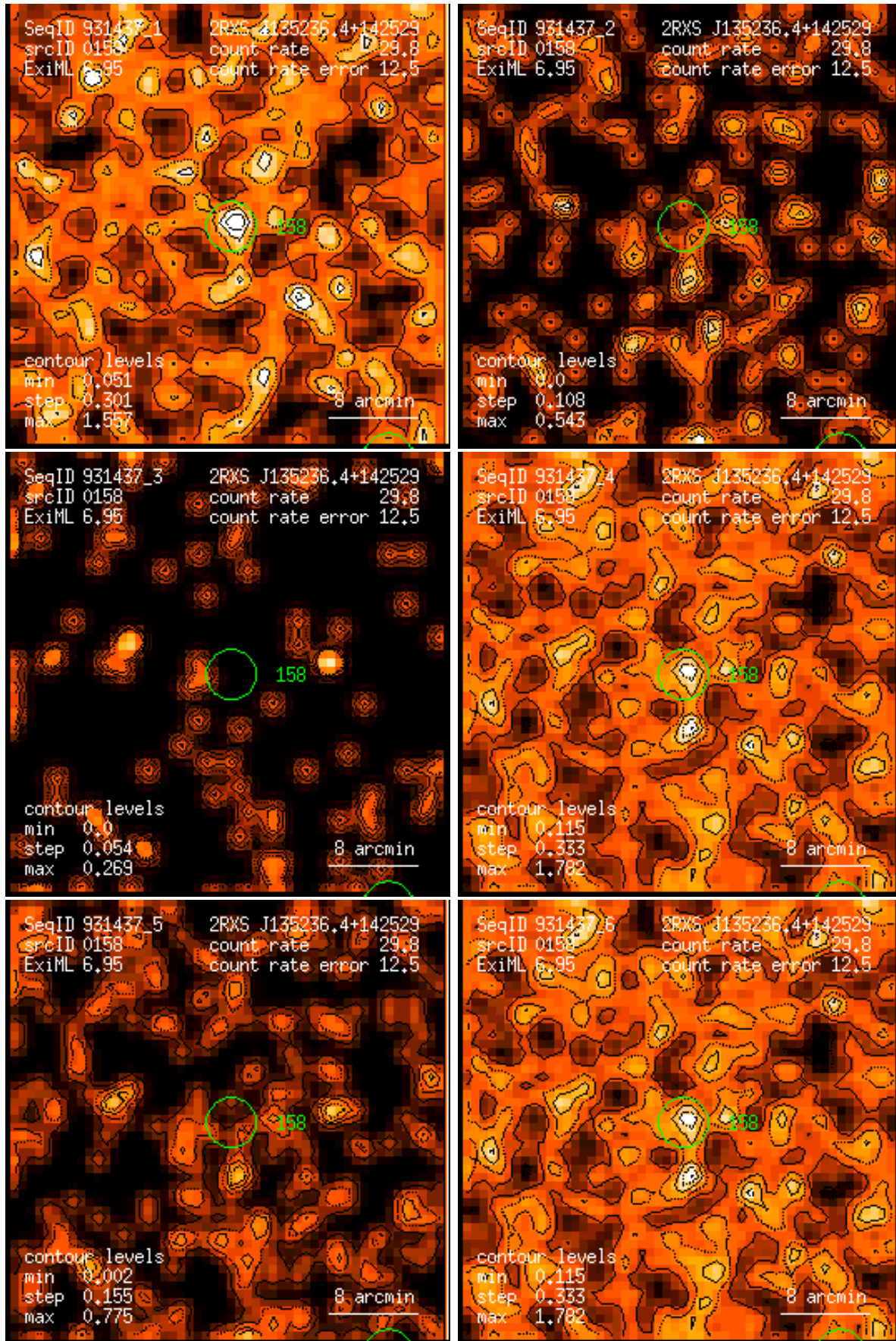
Figure 158: RASS 931437: detection 0158: band rate images, Gaussian filter: (1) PSPC channels 11 – 41, (2) 52 – 90, (3) 91 – 201, (4) 11 – 235, (5) 52 – 201, (6) 11 – 201. Broad band rates in counts/ks. Band rate contour levels in counts/ks/arcmin 2 .
