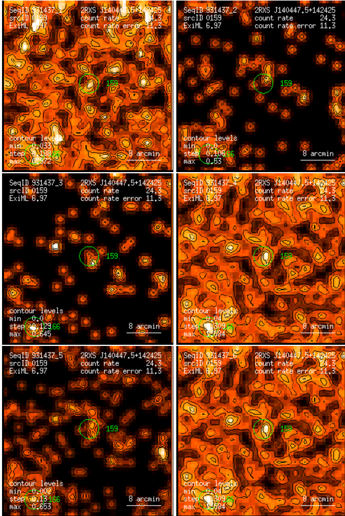
Figure 159: RASS 931437: detection 0159: band rate images, Gaussian filter: (1) PSPC channels 11 – 41, (2) 52 – 90, (3) 91 – 201, (4) 11 – 235, (5) 52 – 201, (6) 11 – 201. Broad band rates in counts/ks. Band rate contour levels in counts/ks/arcmin 2 .
