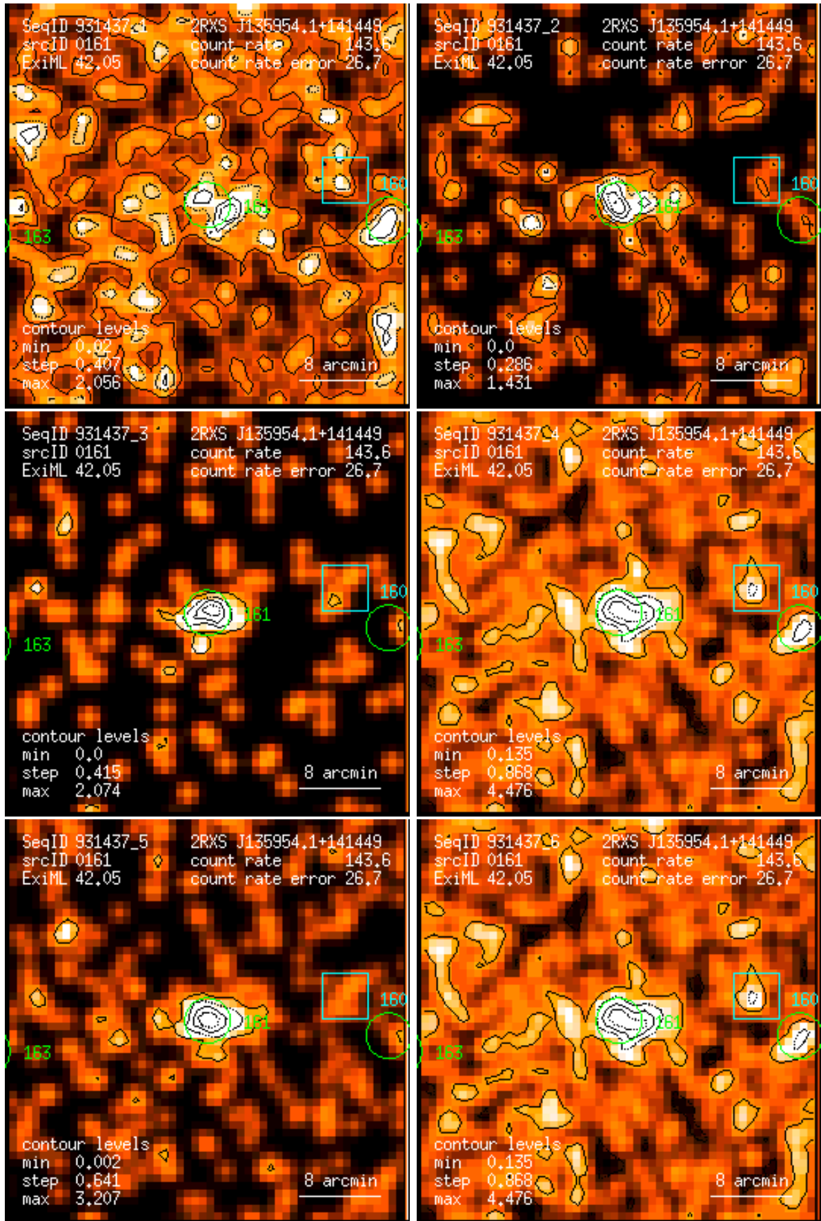
Figure 161: RASS 931437: detection 0161: band rate images, Gaussian filter: (1) PSPC channels 11 – 41, (2) 52 – 90, (3) 91 – 201, (4) 11 – 235, (5) 52 – 201, (6) 11 – 201. Broad band rates in counts/ks. Band rate contour levels in counts/ks/arcmin 2 .
