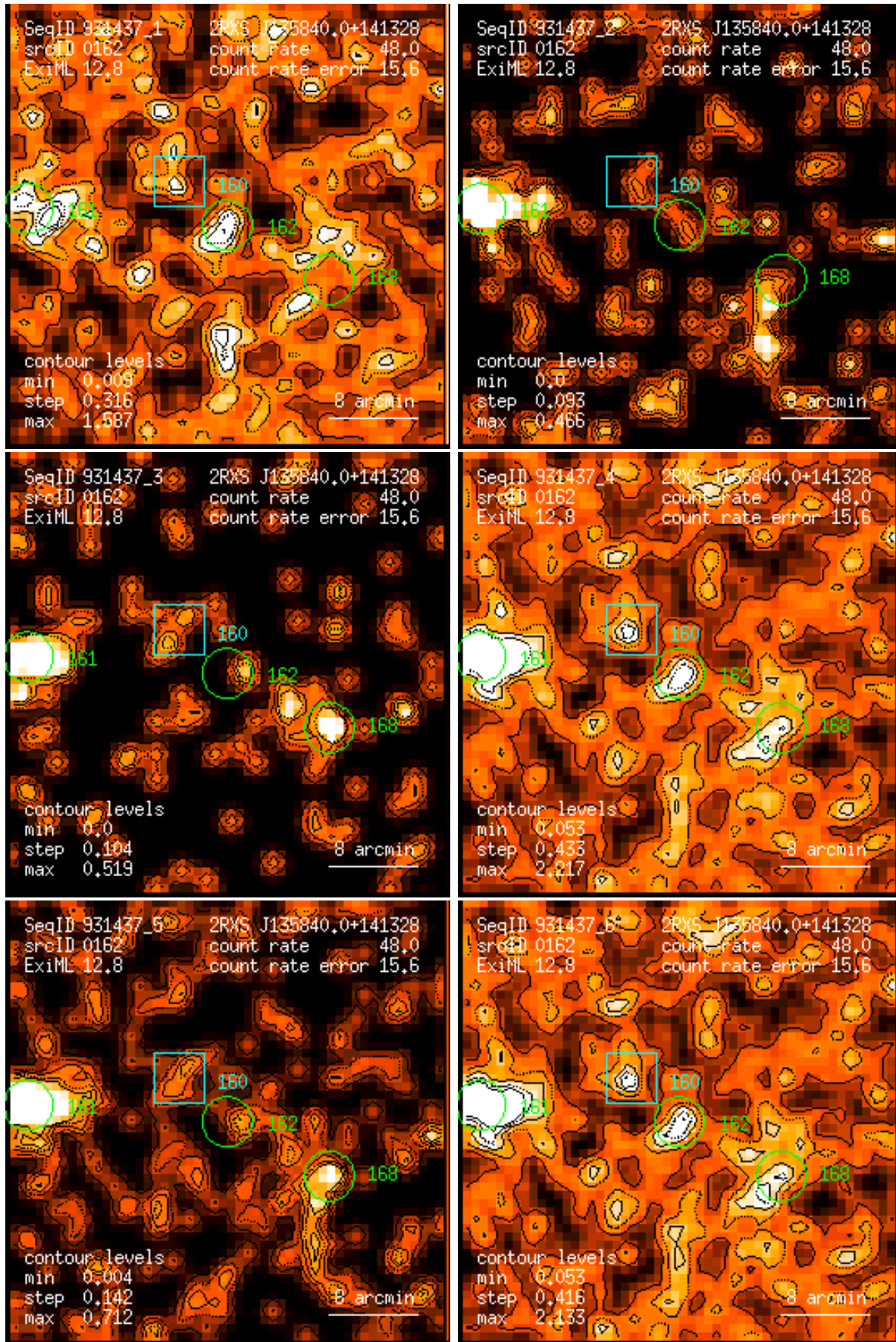
Figure 162: RASS 931437: detection 0162: band rate images, Gaussian filter: (1) PSPC channels 11 – 41, (2) 52 – 90, (3) 91 – 201, (4) 11 – 235, (5) 52 – 201, (6) 11 – 201. Broad band rates in counts/ks. Band rate contour levels in counts/ks/arcmin 2 .
