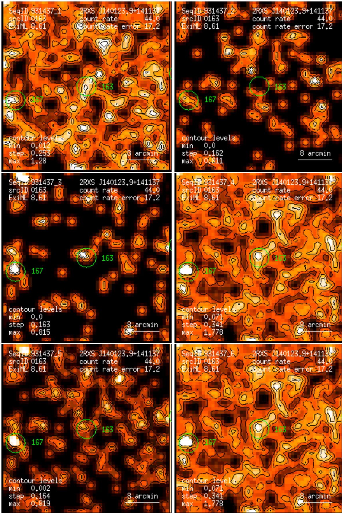
Figure 163: RASS 931437: detection 0163: band rate images, Gaussian filter: (1) PSPC channels 11 – 41, (2) 52 – 90, (3) 91 – 201, (4) 11 – 235, (5) 52 – 201, (6) 11 – 201. Broad band rates in counts/ks. Band rate contour levels in counts/ks/arcmin 2 .
