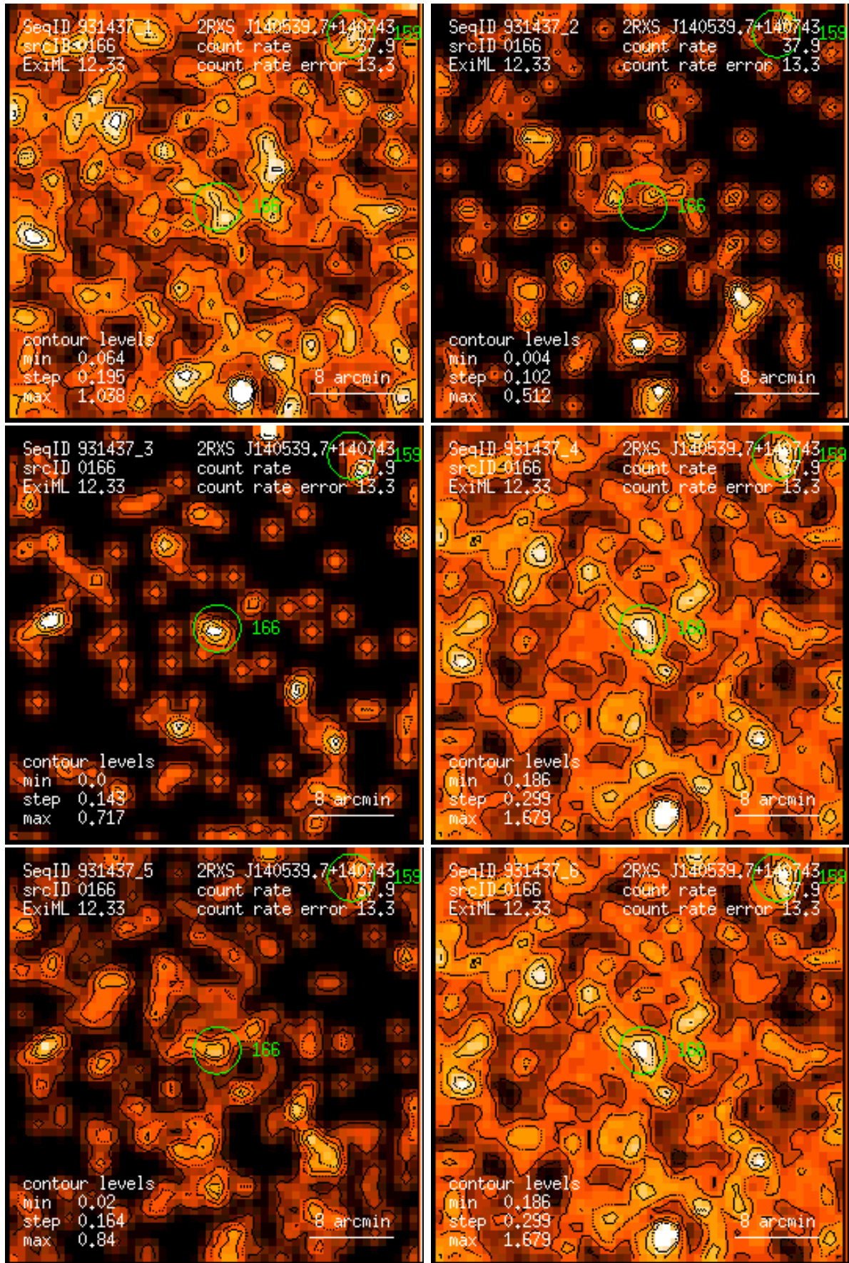
Figure 166: RASS 931437: detection 0166: band rate images, Gaussian filter: (1) PSPC channels 11 – 41, (2) 52 – 90, (3) 91 – 201, (4) 11 – 235, (5) 52 – 201, (6) 11 – 201. Broad band rates in counts/ks. Band rate contour levels in counts/ks/arcmin 2 .
