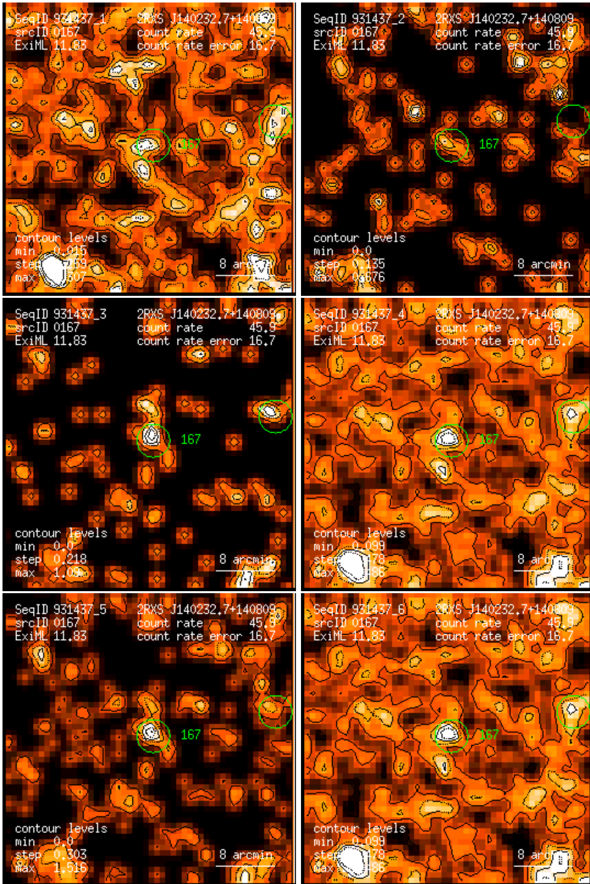
Figure 167: RASS 931437: detection 0167: band rate images, Gaussian filter: (1) PSPC channels 11 – 41, (2) 52 – 90, (3) 91 – 201, (4) 11 – 235, (5) 52 – 201, (6) 11 – 201. Broad band rates in counts/ks. Band rate contour levels in counts/ks/arcmin 2 .
