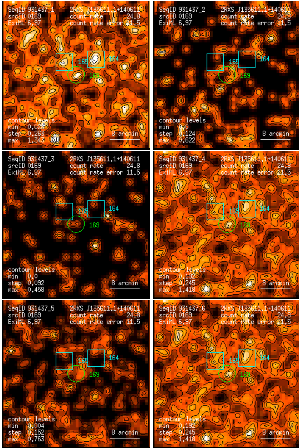
Figure 169: RASS 931437: detection 0169: band rate images, Gaussian filter: (1) PSPC channels 11 – 41, (2) 52 – 90, (3) 91 – 201, (4) 11 – 235, (5) 52 – 201, (6) 11 – 201. Broad band rates in counts/ks. Band rate contour levels in counts/ks/arcmin 2 .
