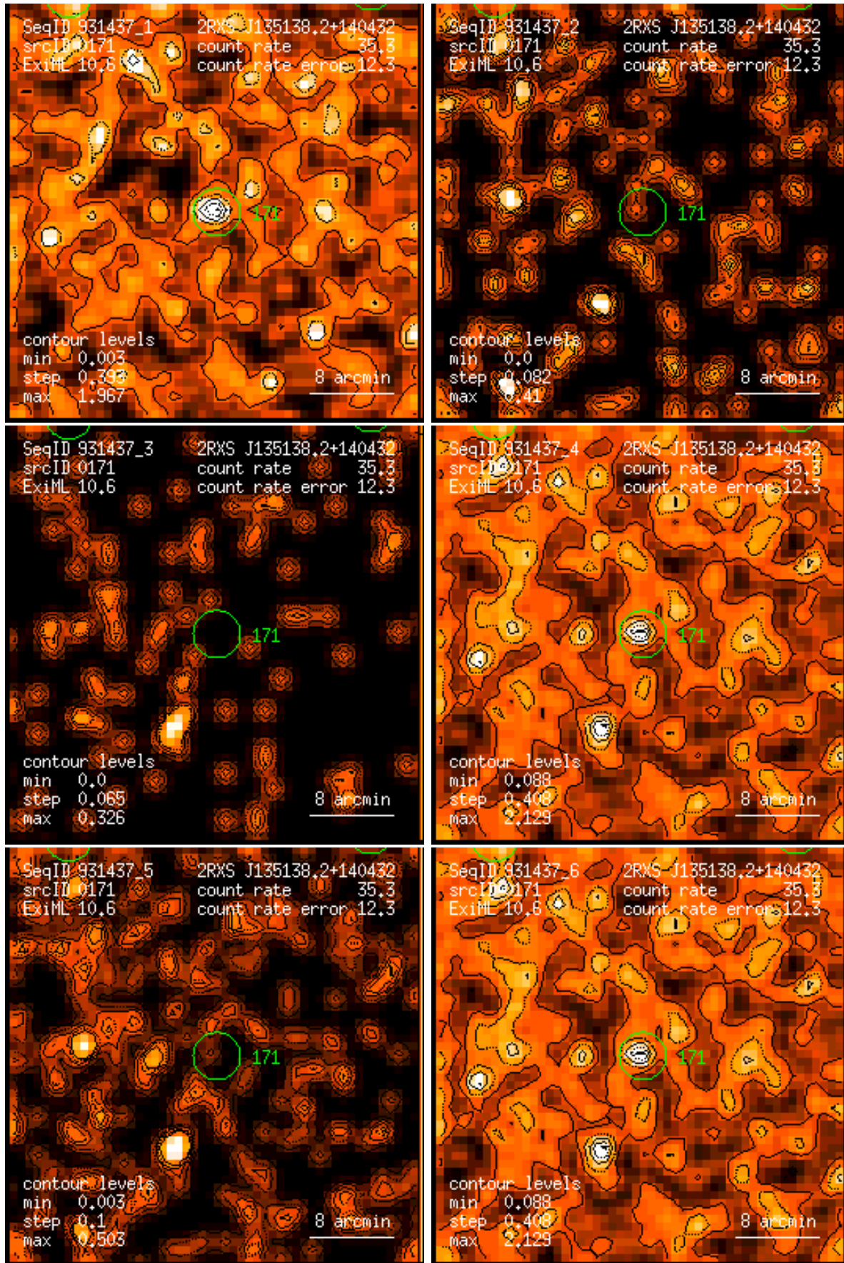
Figure 171: RASS 931437: detection 0171: band rate images, Gaussian filter: (1) PSPC channels 11 – 41, (2) 52 – 90, (3) 91 – 201, (4) 11 – 235, (5) 52 – 201, (6) 11 – 201. Broad band rates in counts/ks. Band rate contour levels in counts/ks/arcmin 2 .
