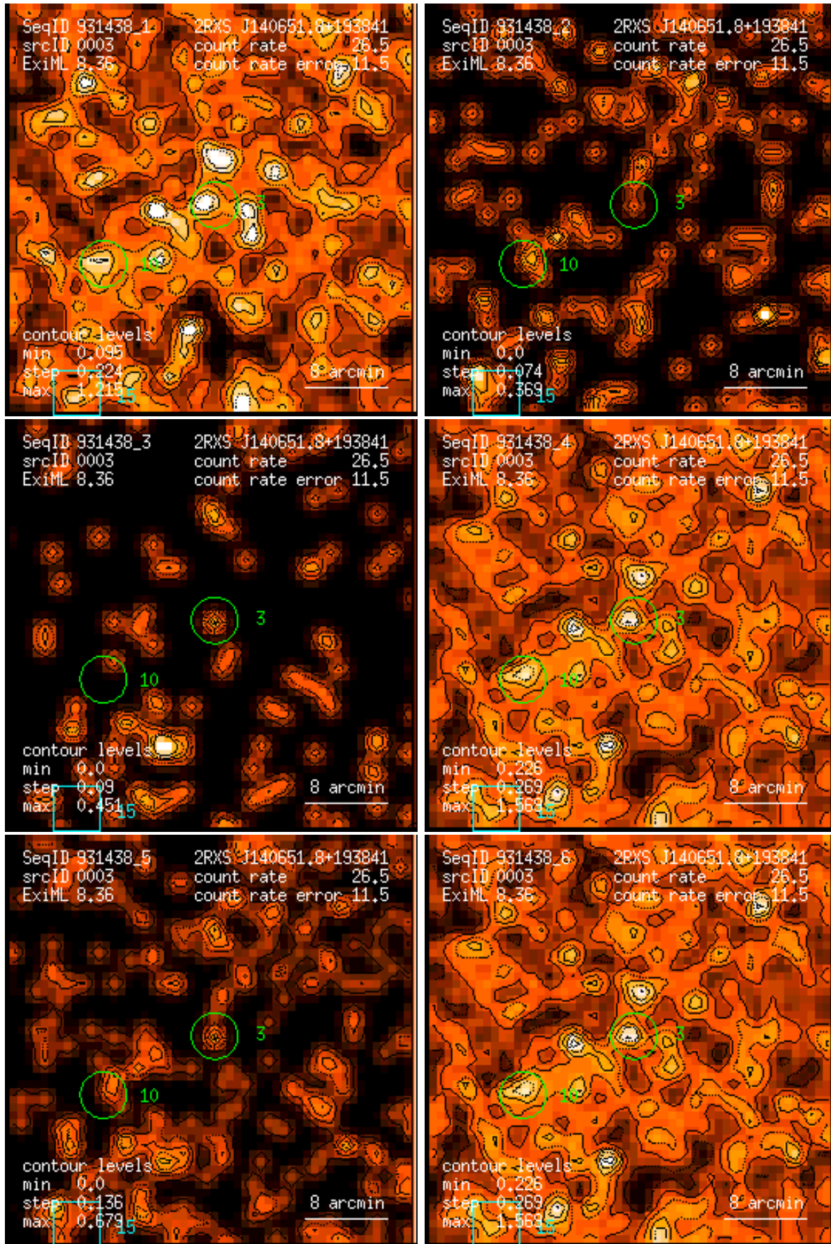
Figure 3: RASS 931438: detection 0003: band rate images, Gaussian filter: (1) PSPC channels 11 – 41, (2) 52 – 90, (3) 91 – 201, (4) 11 – 235, (5) 52 – 201, (6) 11 – 201. Broad band rates in counts/ks. Band rate contour levels in counts/ks/arcmin 2 .
