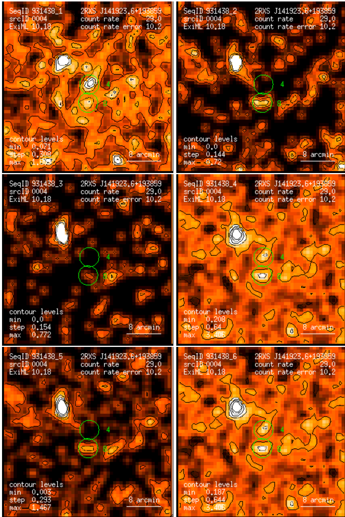
Figure 4: RASS 931438: detection 0004: band rate images, Gaussian filter: (1) PSPC channels 11 – 41, (2) 52 – 90, (3) 91 – 201, (4) 11 – 235, (5) 52 – 201, (6) 11 – 201. Broad band rates in counts/ks. Band rate contour levels in counts/ks/arcmin 2 .
