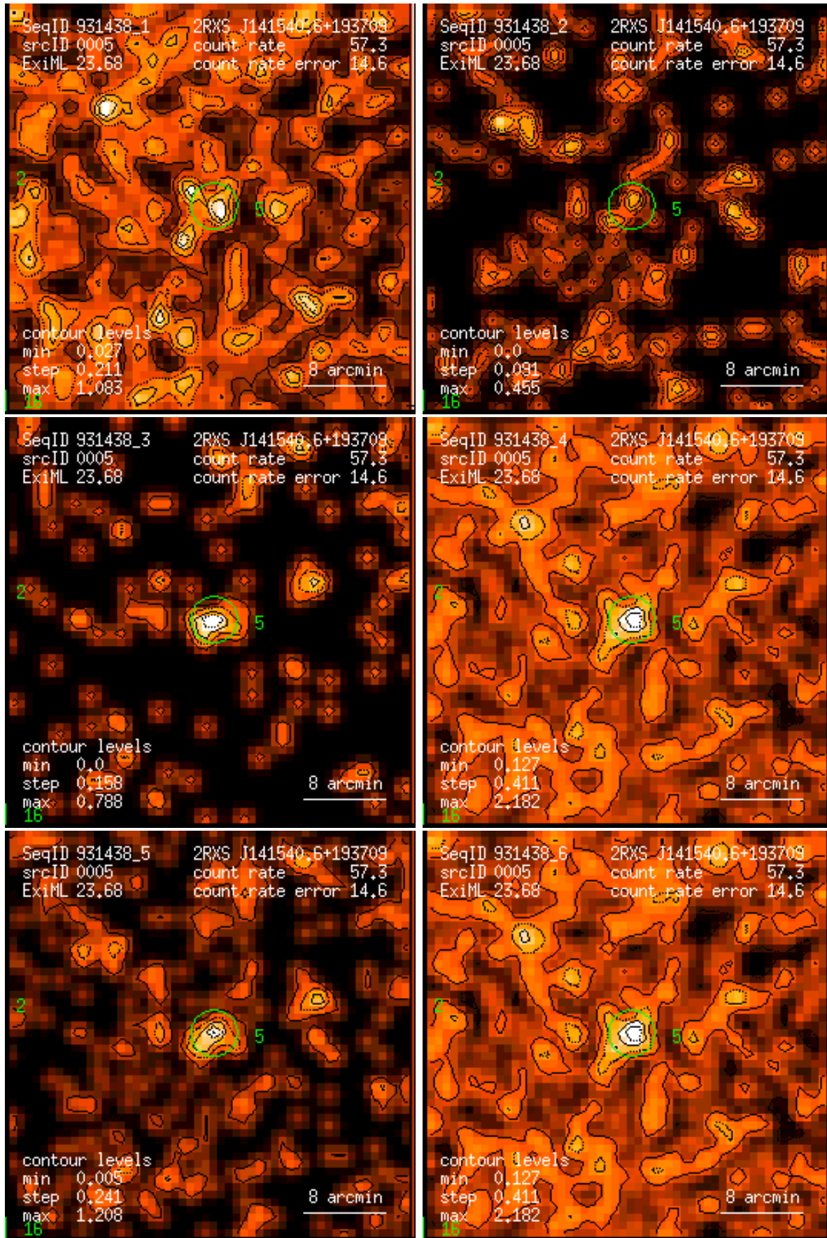
Figure 5: RASS 931438: detection 0005: band rate images, Gaussian filter: (1) PSPC channels 11 – 41, (2) 52 – 90, (3) 91 – 201, (4) 11 – 235, (5) 52 – 201, (6) 11 – 201. Broad band rates in counts/ks. Band rate contour levels in counts/ks/arcmin 2 .
