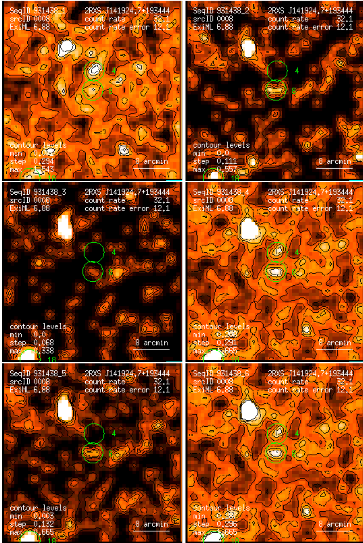
Figure 8: RASS 931438: detection 0008: band rate images, Gaussian filter: (1) PSPC channels 11 – 41, (2) 52 – 90, (3) 91 – 201, (4) 11 – 235, (5) 52 – 201, (6) 11 – 201. Broad band rates in counts/ks. Band rate contour levels in counts/ks/arcmin 2 .
