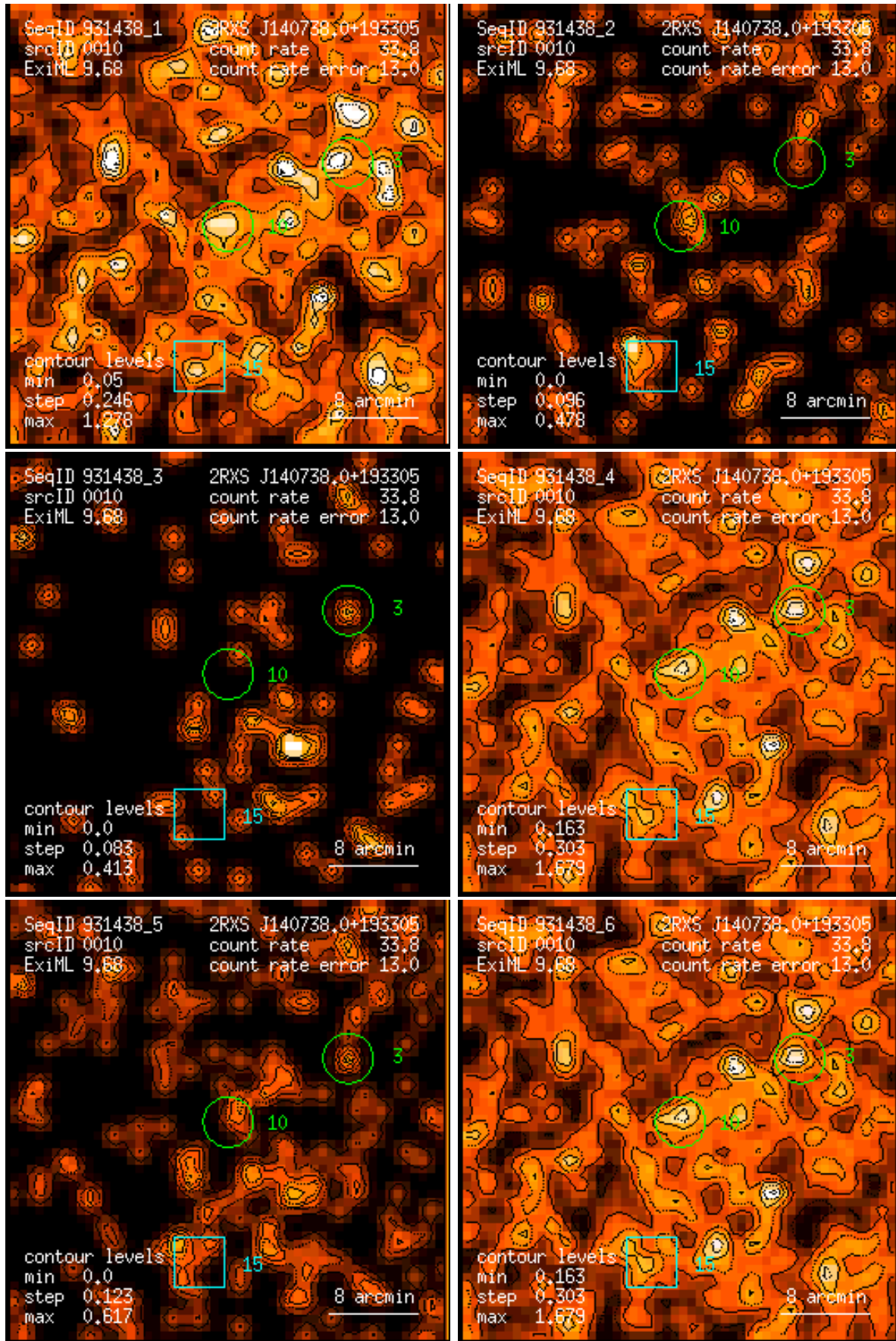
Figure 10: RASS 931438: detection 0010: band rate images, Gaussian filter: (1) PSPC channels 11 – 41, (2) 52 – 90, (3) 91 – 201, (4) 11 – 235, (5) 52 – 201, (6) 11 – 201. Broad band rates in counts/ks. Band rate contour levels in counts/ks/arcmin 2 .
