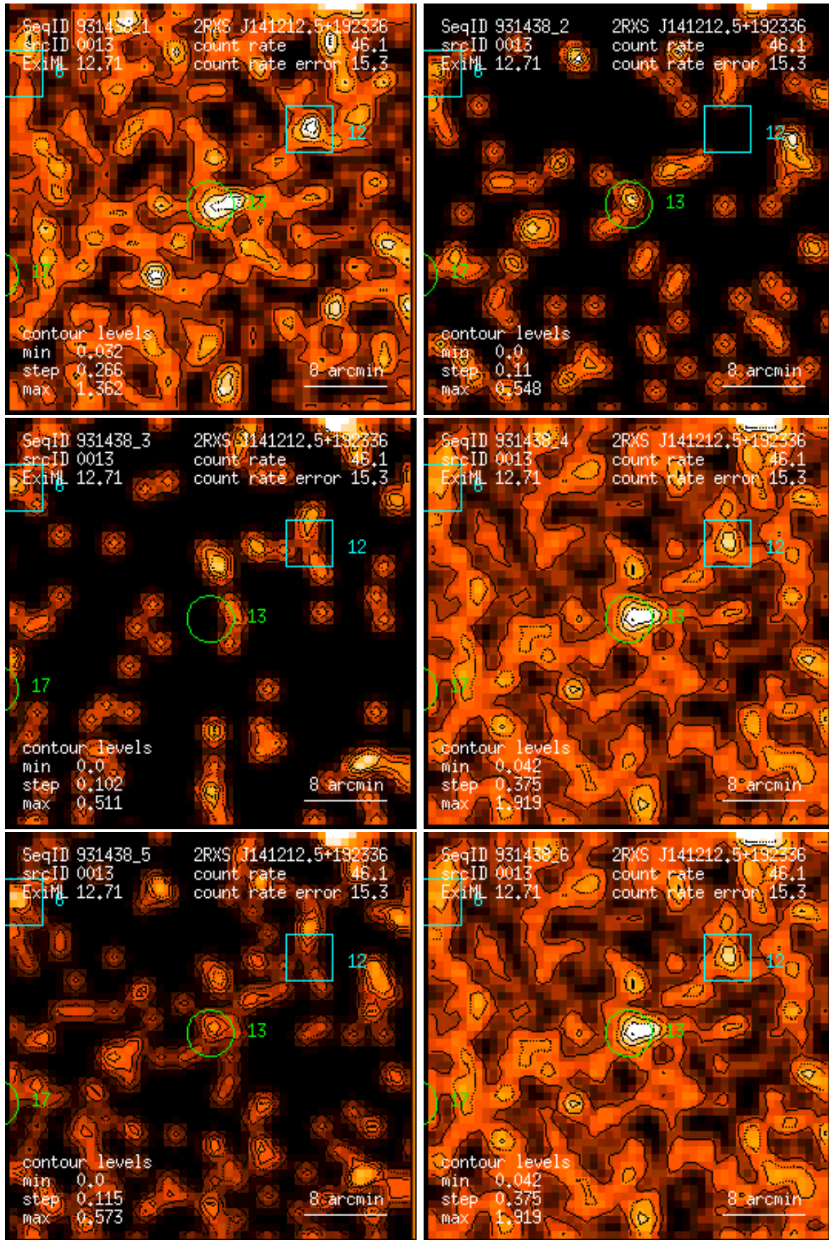
Figure 13: RASS 931438: detection 0013: band rate images, Gaussian filter: (1) PSPC channels 11 – 41, (2) 52 – 90, (3) 91 – 201, (4) 11 – 235, (5) 52 – 201, (6) 11 – 201. Broad band rates in counts/ks. Band rate contour levels in counts/ks/arcmin 2 .
