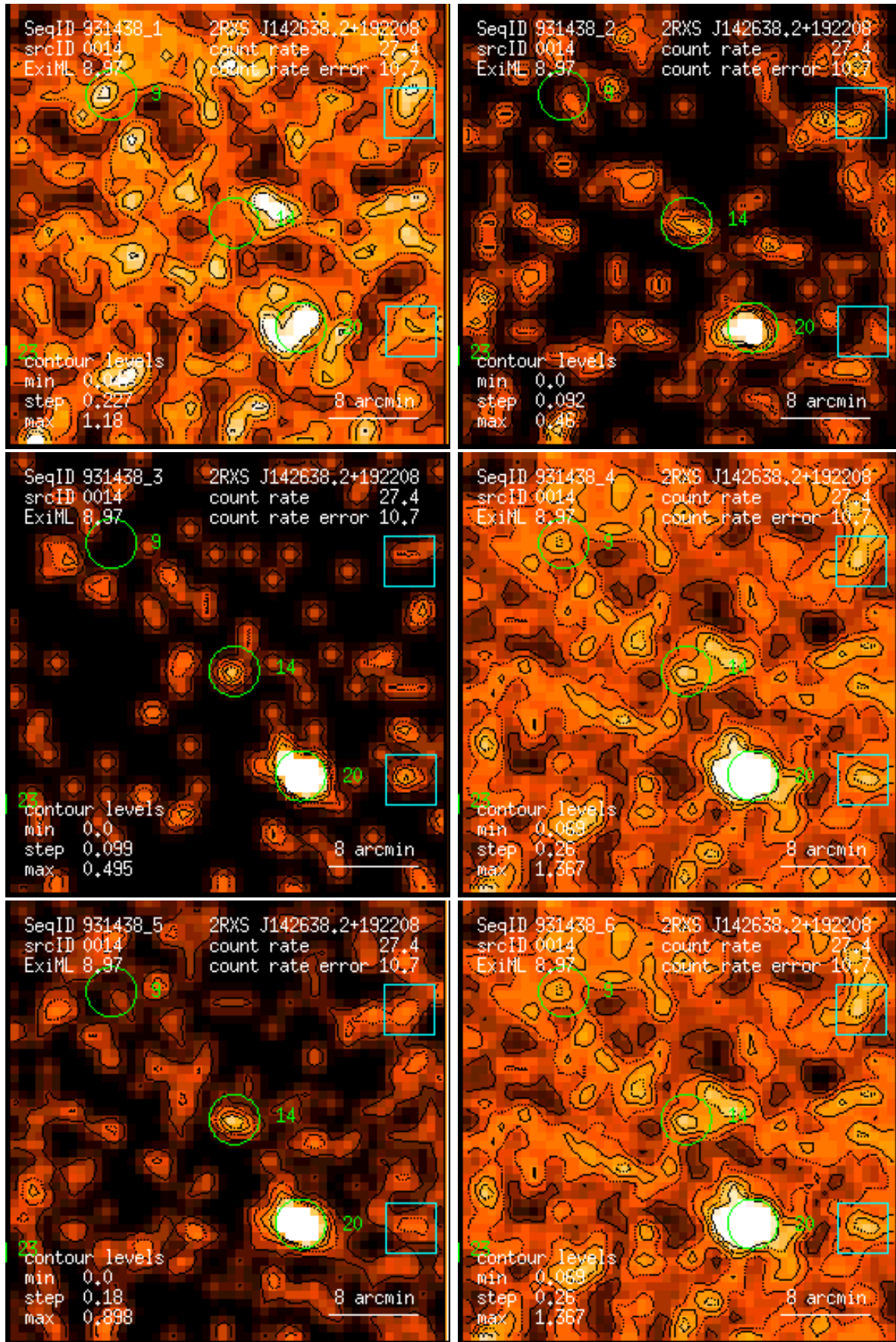
Figure 14: RASS 931438: detection 0014: band rate images, Gaussian filter: (1) PSPC channels 11 – 41, (2) 52 – 90, (3) 91 – 201, (4) 11 – 235, (5) 52 – 201, (6) 11 – 201. Broad band rates in counts/ks. Band rate contour levels in counts/ks/arcmin 2 .
