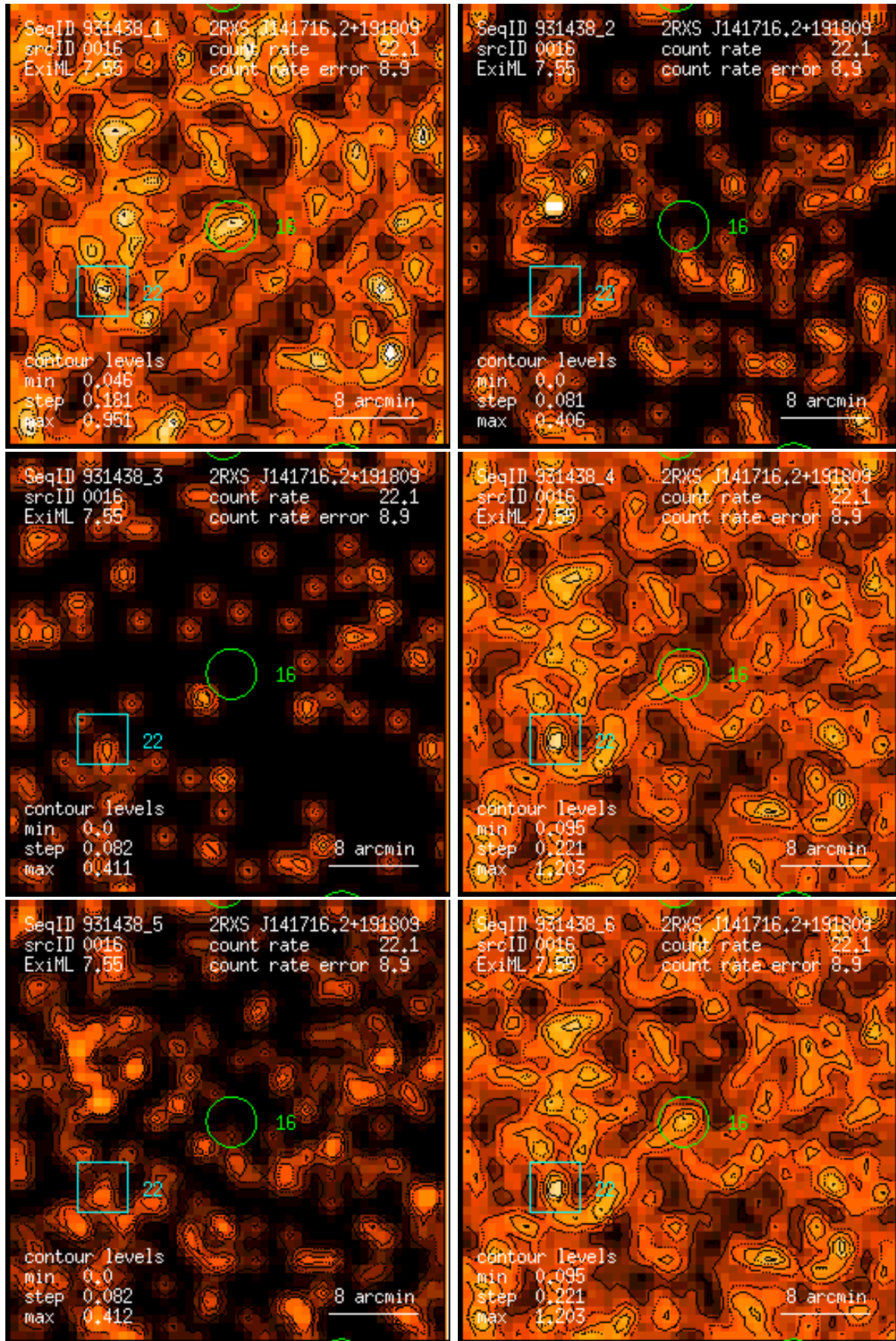
Figure 16: RASS 931438: detection 0016: band rate images, Gaussian filter: (1) PSPC channels 11 – 41, (2) 52 – 90, (3) 91 – 201, (4) 11 – 235, (5) 52 – 201, (6) 11 – 201. Broad band rates in counts/ks. Band rate contour levels in counts/ks/arcmin 2 .
