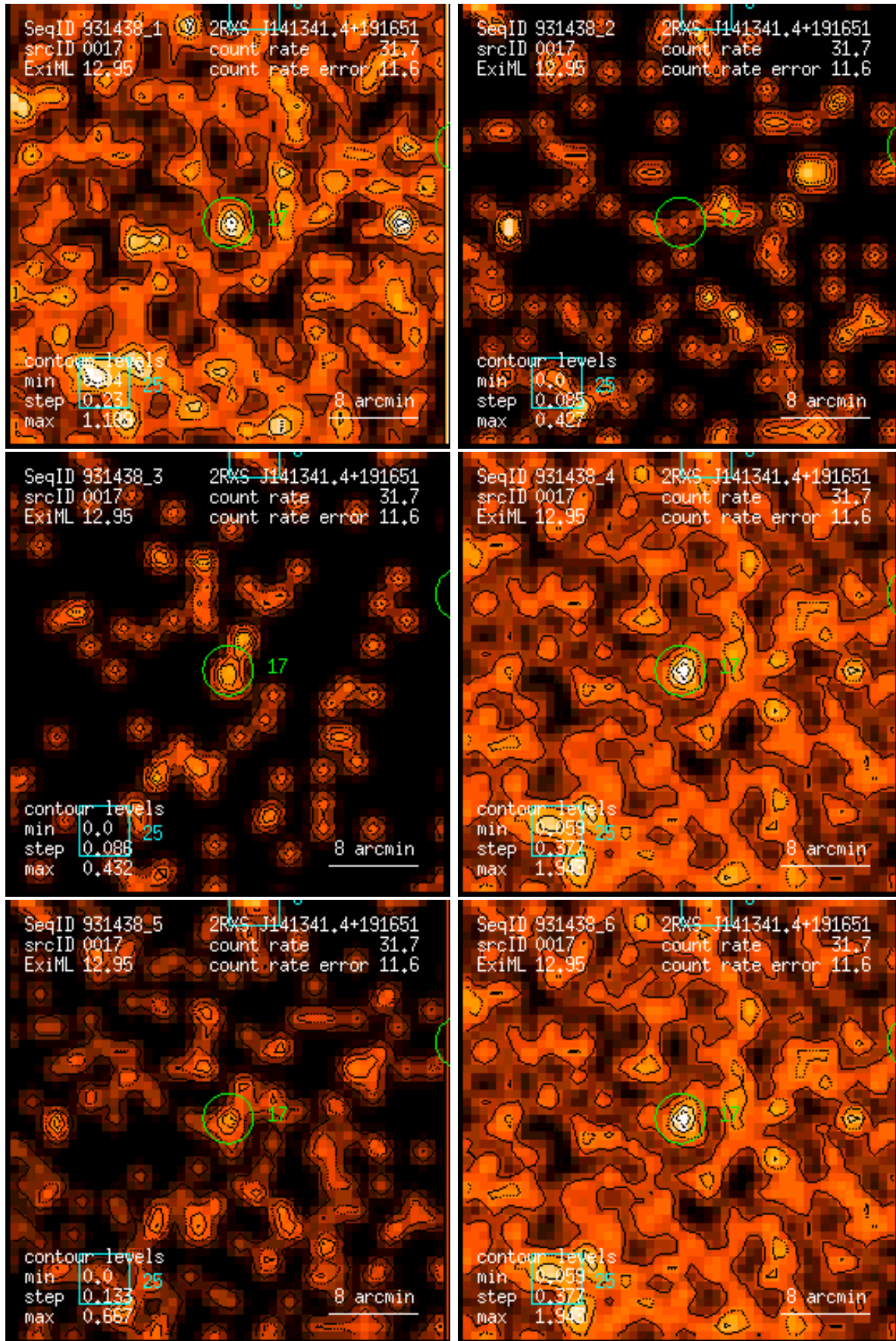
Figure 17: RASS 931438: detection 0017: band rate images, Gaussian filter: (1) PSPC channels 11 – 41, (2) 52 – 90, (3) 91 – 201, (4) 11 – 235, (5) 52 – 201, (6) 11 – 201. Broad band rates in counts/ks. Band rate contour levels in counts/ks/arcmin 2 .
