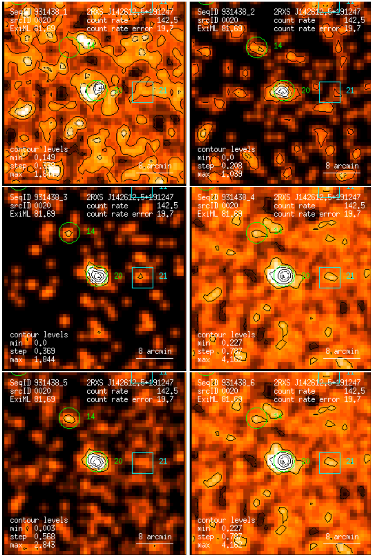
Figure 20: RASS 931438: detection 0020: band rate images, Gaussian filter: (1) PSPC channels 11 – 41, (2) 52 – 90, (3) 91 – 201, (4) 11 – 235, (5) 52 – 201, (6) 11 – 201. Broad band rates in counts/ks. Band rate contour levels in counts/ks/arcmin 2 .
