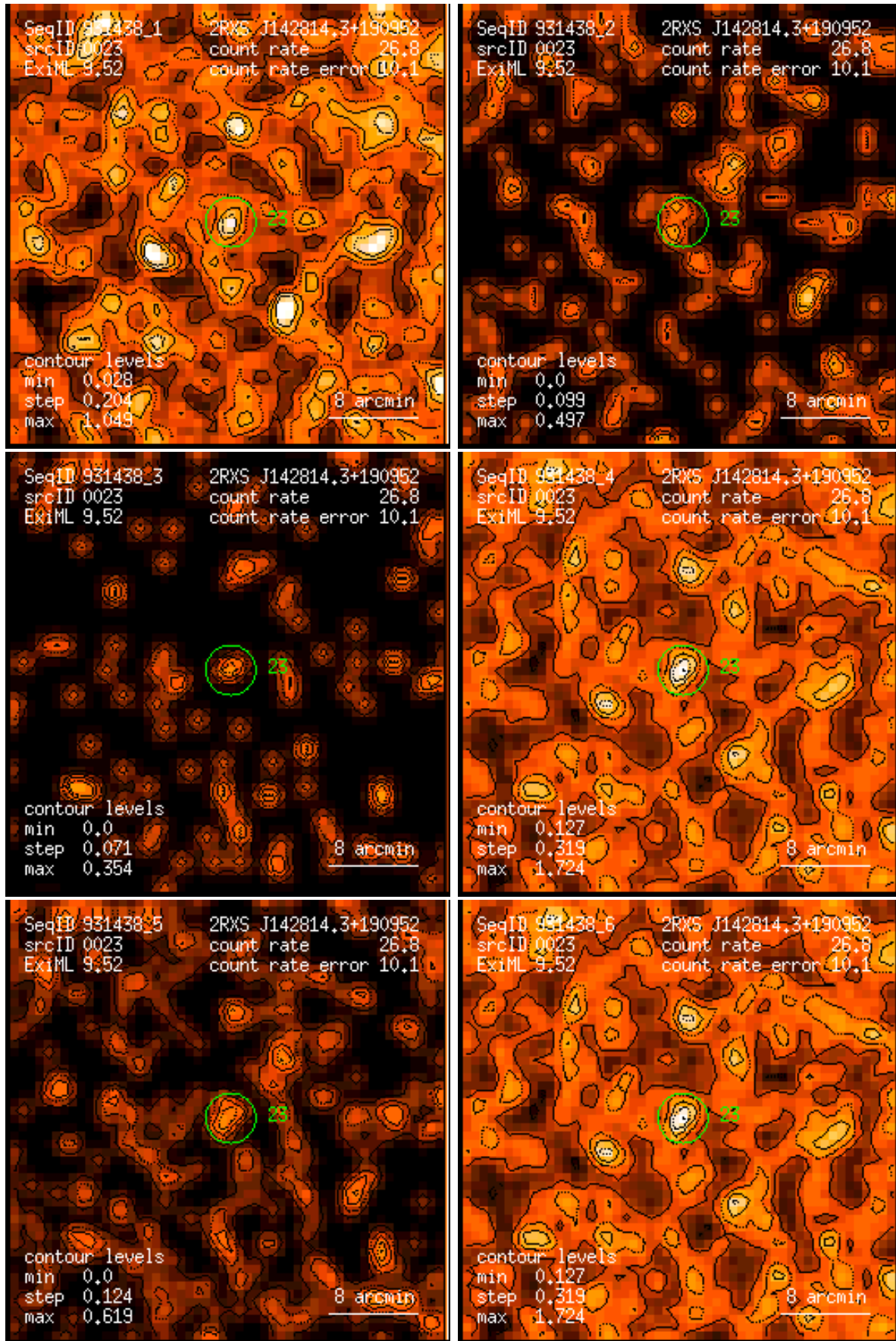
Figure 23: RASS 931438: detection 0023: band rate images, Gaussian filter: (1) PSPC channels 11 – 41, (2) 52 – 90, (3) 91 – 201, (4) 11 – 235, (5) 52 – 201, (6) 11 – 201. Broad band rates in counts/ks. Band rate contour levels in counts/ks/arcmin 2 .
