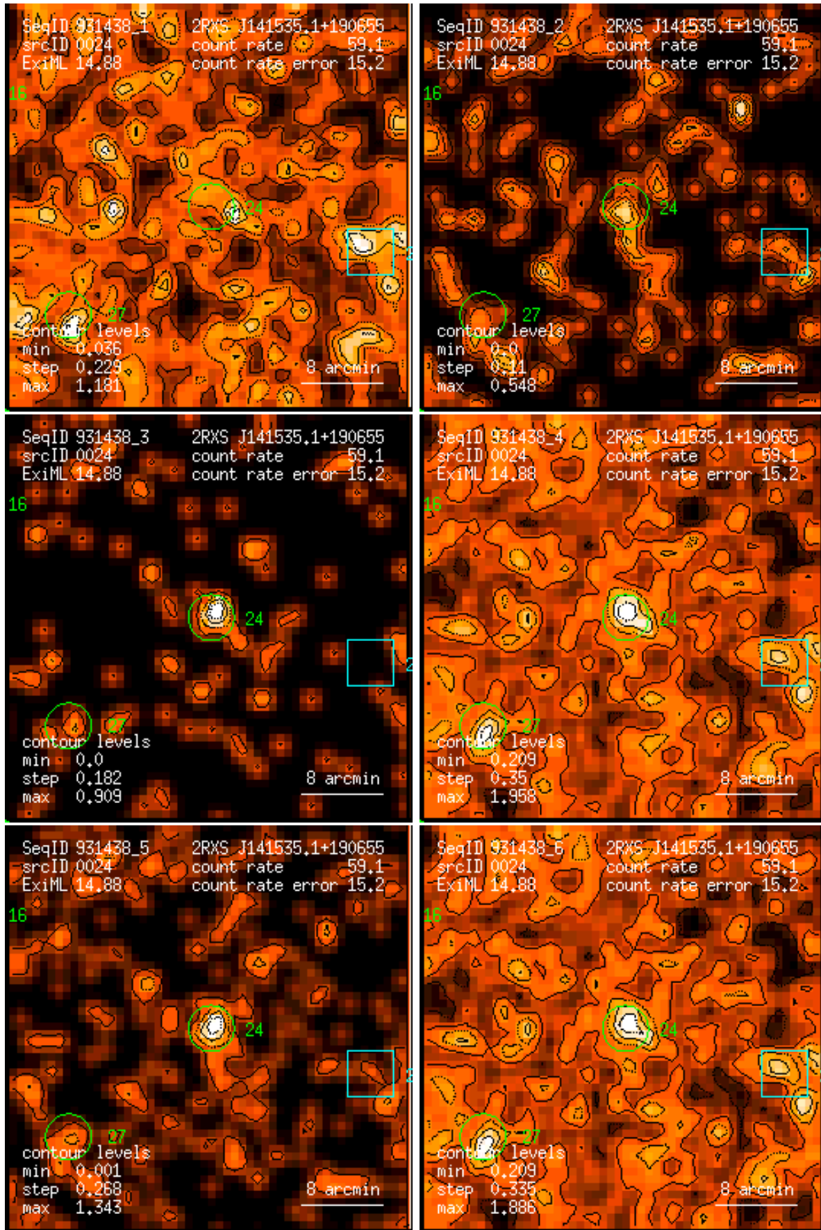
Figure 24: RASS 931438: detection 0024: band rate images, Gaussian filter: (1) PSPC channels 11 – 41, (2) 52 – 90, (3) 91 – 201, (4) 11 – 235, (5) 52 – 201, (6) 11 – 201. Broad band rates in counts/ks. Band rate contour levels in counts/ks/arcmin 2 .
