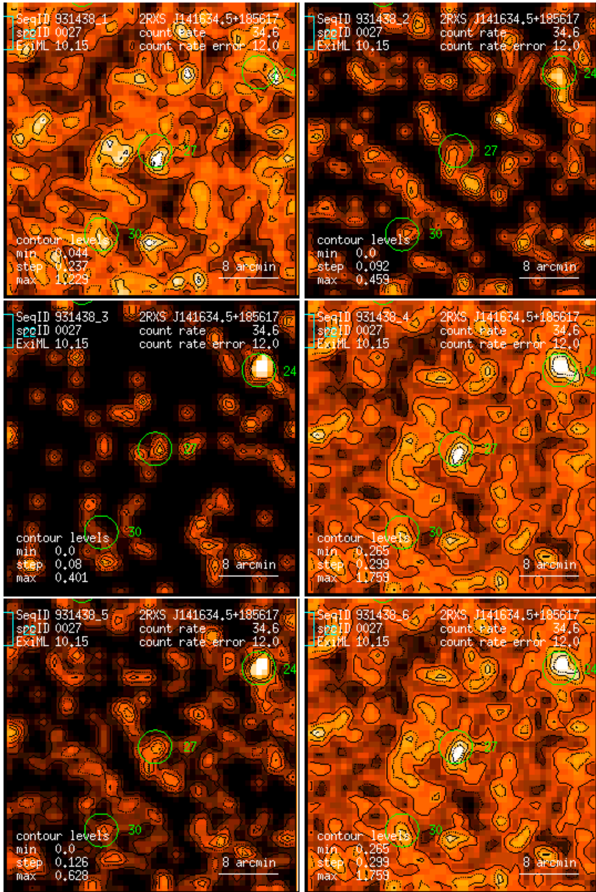
Figure 27: RASS 931438: detection 0027: band rate images, Gaussian filter: (1) PSPC channels 11 – 41, (2) 52 – 90, (3) 91 – 201, (4) 11 – 235, (5) 52 – 201, (6) 11 – 201. Broad band rates in counts/ks. Band rate contour levels in counts/ks/arcmin 2 .
