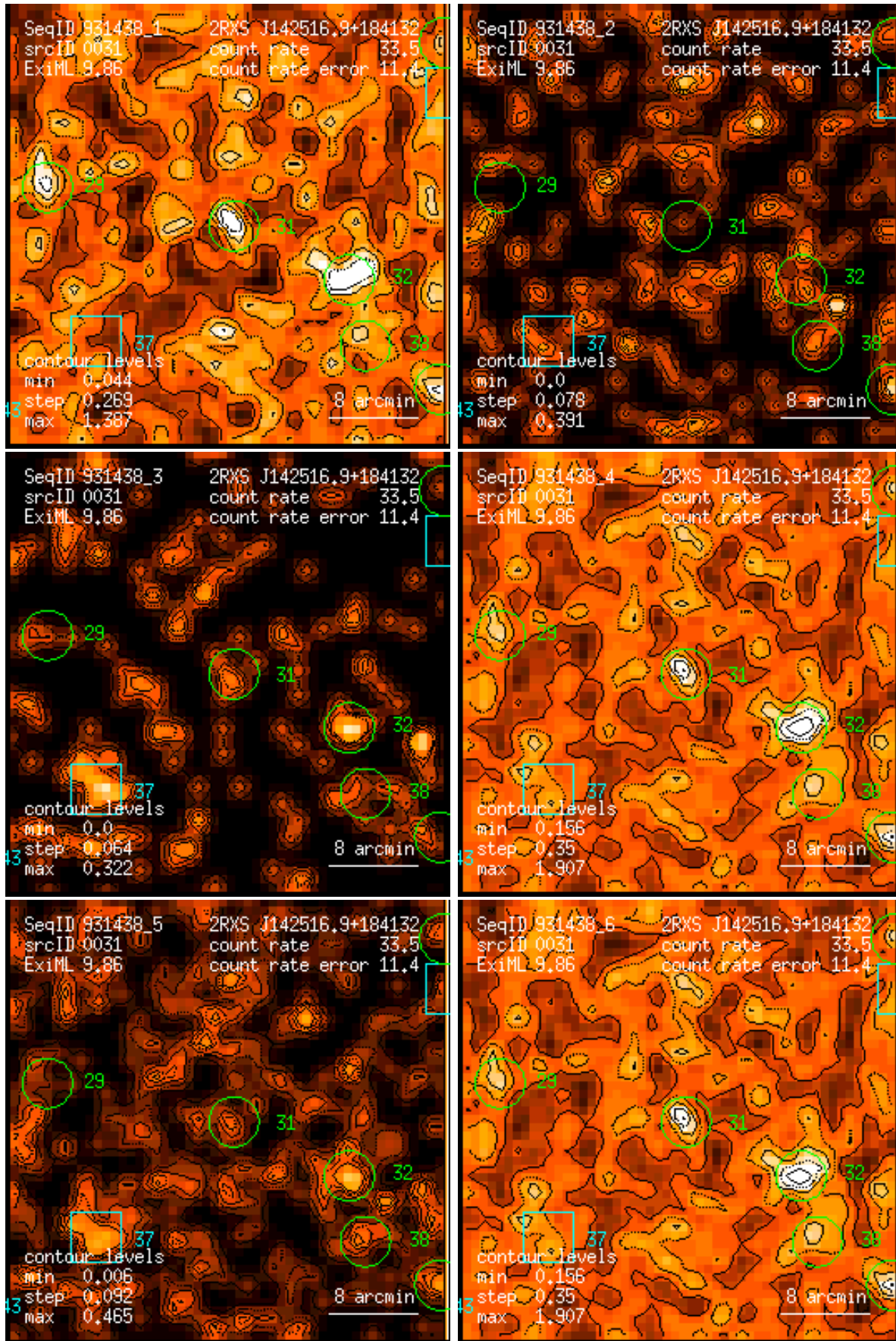
Figure 31: RASS 931438: detection 0031: band rate images, Gaussian filter: (1) PSPC channels 11 – 41, (2) 52 – 90, (3) 91 – 201, (4) 11 – 235, (5) 52 – 201, (6) 11 – 201. Broad band rates in counts/ks. Band rate contour levels in counts/ks/arcmin 2 .
