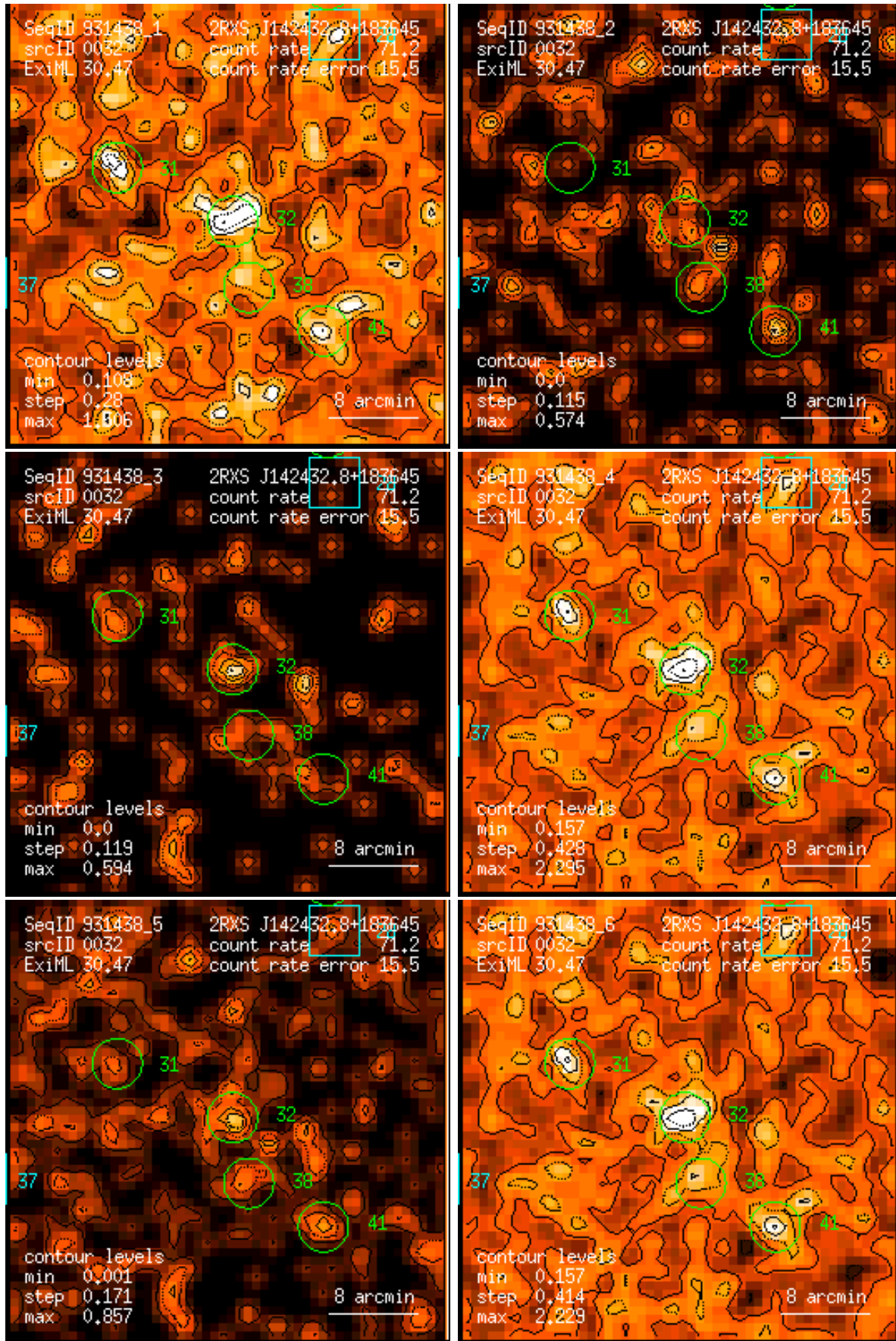
Figure 32: RASS 931438: detection 0032: band rate images, Gaussian filter: (1) PSPC channels 11 – 41, (2) 52 – 90, (3) 91 – 201, (4) 11 – 235, (5) 52 – 201, (6) 11 – 201. Broad band rates in counts/ks. Band rate contour levels in counts/ks/arcmin 2 .
