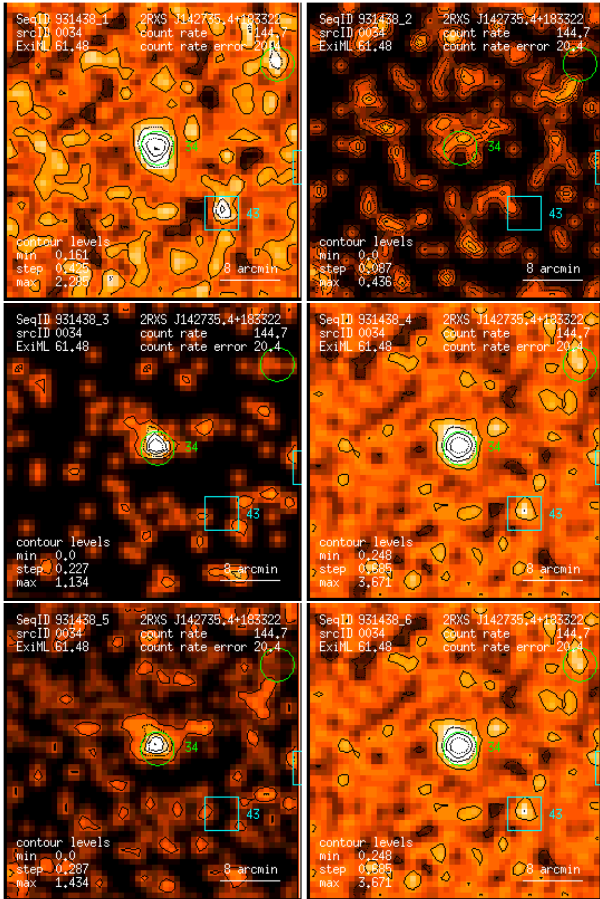
Figure 34: RASS 931438: detection 0034: band rate images, Gaussian filter: (1) PSPC channels 11 – 41, (2) 52 – 90, (3) 91 – 201, (4) 11 – 235, (5) 52 – 201, (6) 11 – 201. Broad band rates in counts/ks. Band rate contour levels in counts/ks/arcmin 2 .
