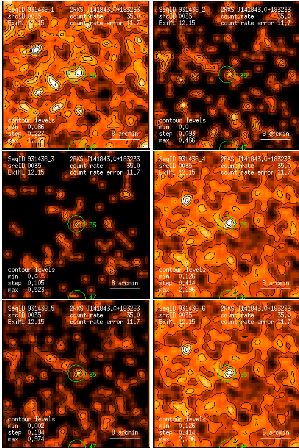
Figure 35: RASS 931438: detection 0035: band rate images, Gaussian filter: (1) PSPC channels 11 – 41, (2) 52 – 90, (3) 91 – 201, (4) 11 – 235, (5) 52 – 201, (6) 11 – 201. Broad band rates in counts/ks. Band rate contour levels in counts/ks/arcmin 2 .
