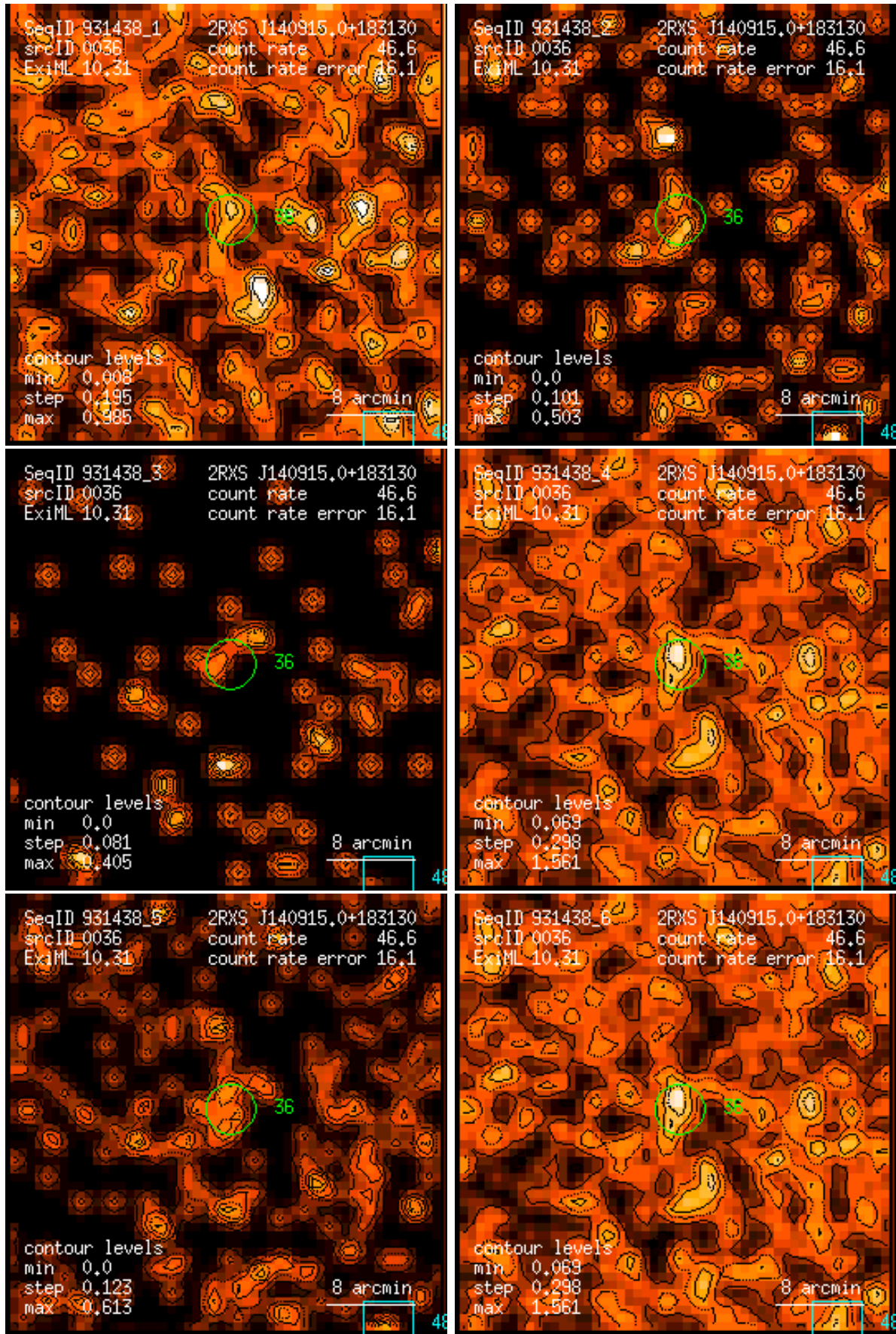
Figure 36: RASS 931438: detection 0036: band rate images, Gaussian filter: (1) PSPC channels 11 – 41, (2) 52 – 90, (3) 91 – 201, (4) 11 – 235, (5) 52 – 201, (6) 11 – 201. Broad band rates in counts/ks. Band rate contour levels in counts/ks/arcmin 2 .
