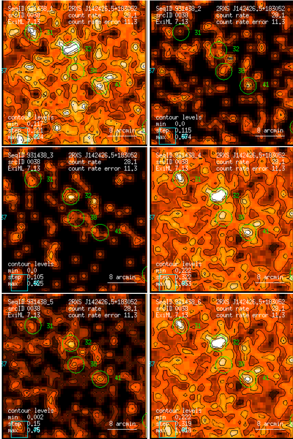
Figure 38: RASS 931438: detection 0038: band rate images, Gaussian filter: (1) PSPC channels 11 – 41, (2) 52 – 90, (3) 91 – 201, (4) 11 – 235, (5) 52 – 201, (6) 11 – 201. Broad band rates in counts/ks. Band rate contour levels in counts/ks/arcmin 2 .
