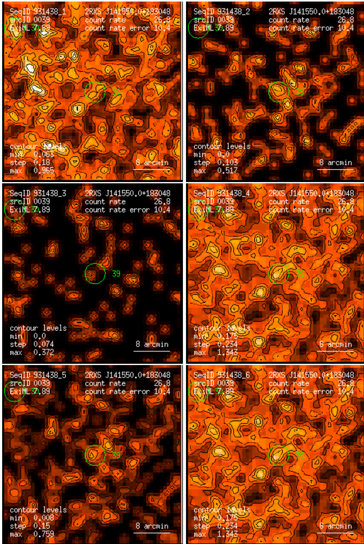
Figure 39: RASS 931438: detection 0039: band rate images, Gaussian filter: (1) PSPC channels 11 – 41, (2) 52 – 90, (3) 91 – 201, (4) 11 – 235, (5) 52 – 201, (6) 11 – 201. Broad band rates in counts/ks. Band rate contour levels in counts/ks/arcmin 2 .
