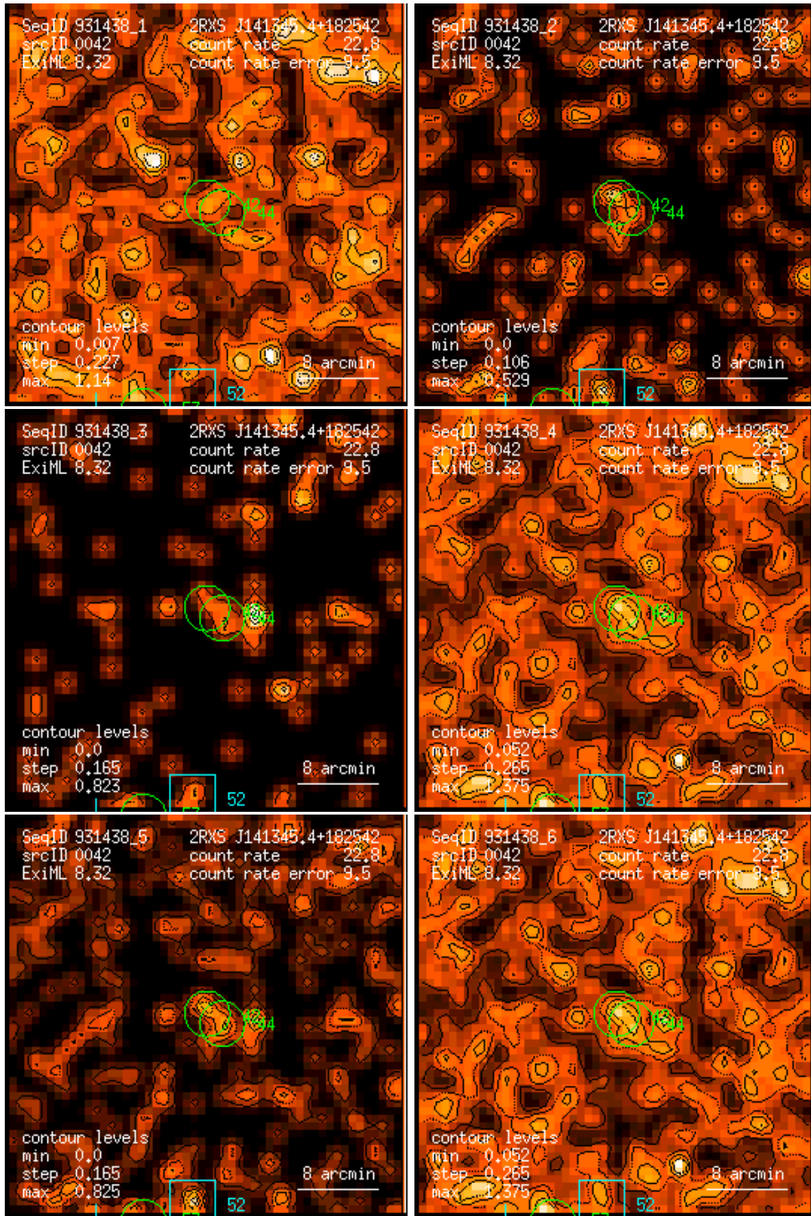
Figure 42: RASS 931438: detection 0042: band rate images, Gaussian filter: (1) PSPC channels 11 – 41, (2) 52 – 90, (3) 91 – 201, (4) 11 – 235, (5) 52 – 201, (6) 11 – 201. Broad band rates in counts/ks. Band rate contour levels in counts/ks/arcmin 2 .
